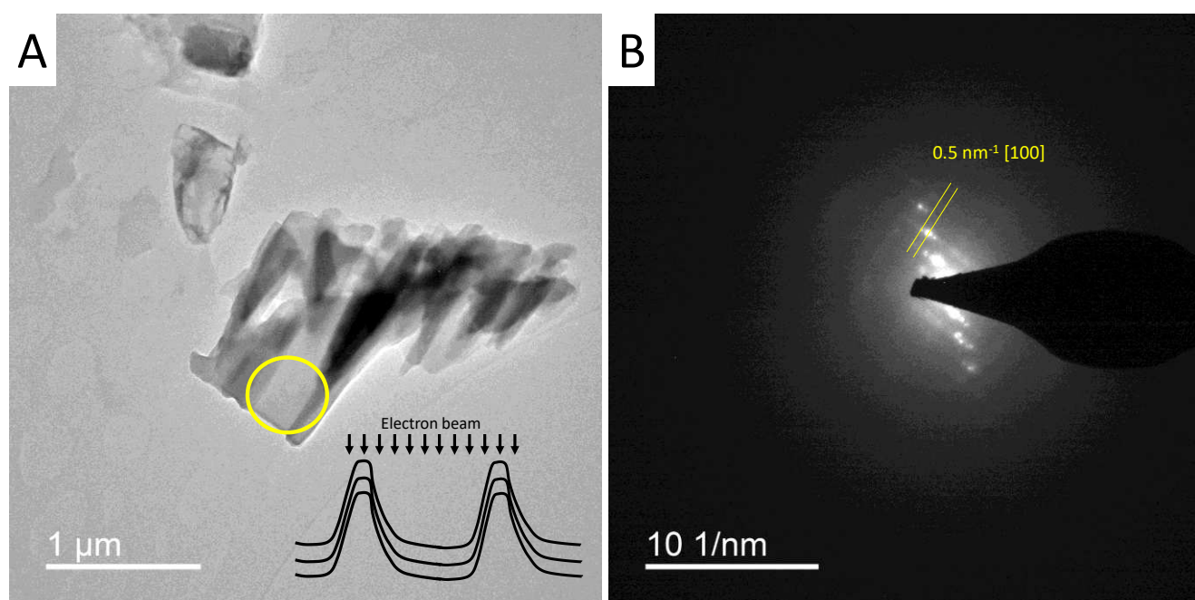
Figure 28: A) TEM analysis of CTF-2D material. Yellow circle: SAED analysed area. Insert: model of the analysed area; B) corresponding SAED analysis.
