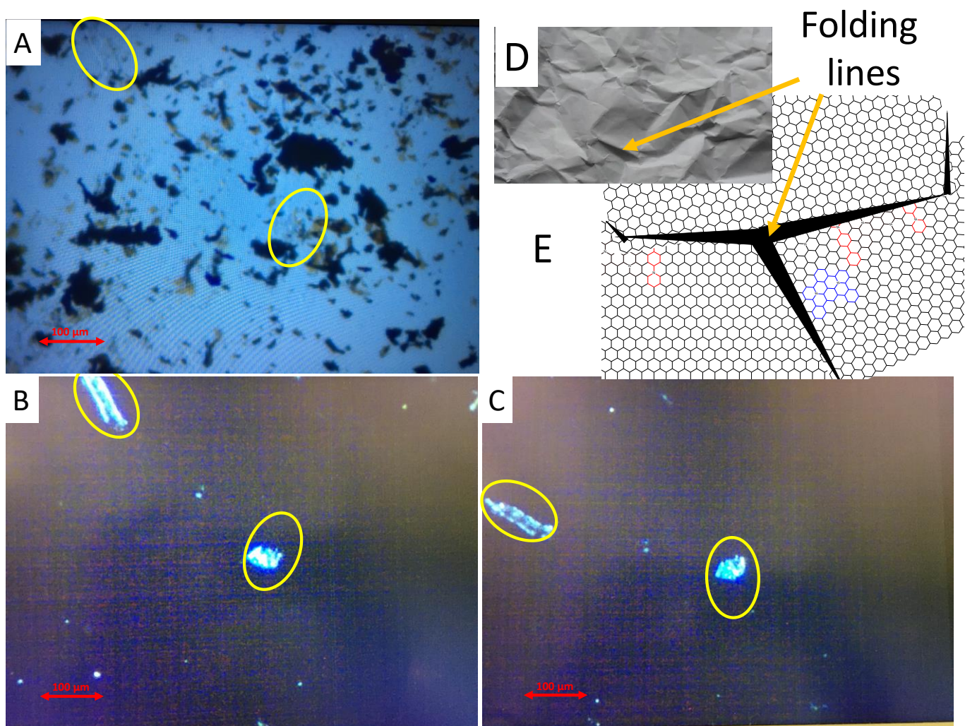
Figure 15: polarised light study of thin C_2N flakes (yellow circles). A): normal light; B): same flakes under cross polarized light and C) same sample upon rotation. The appearance of the flakes alternatively goes brighter and darker as a function of the angle. D) and E): a simple model accounting for the observation of different domains inside a single flake.
