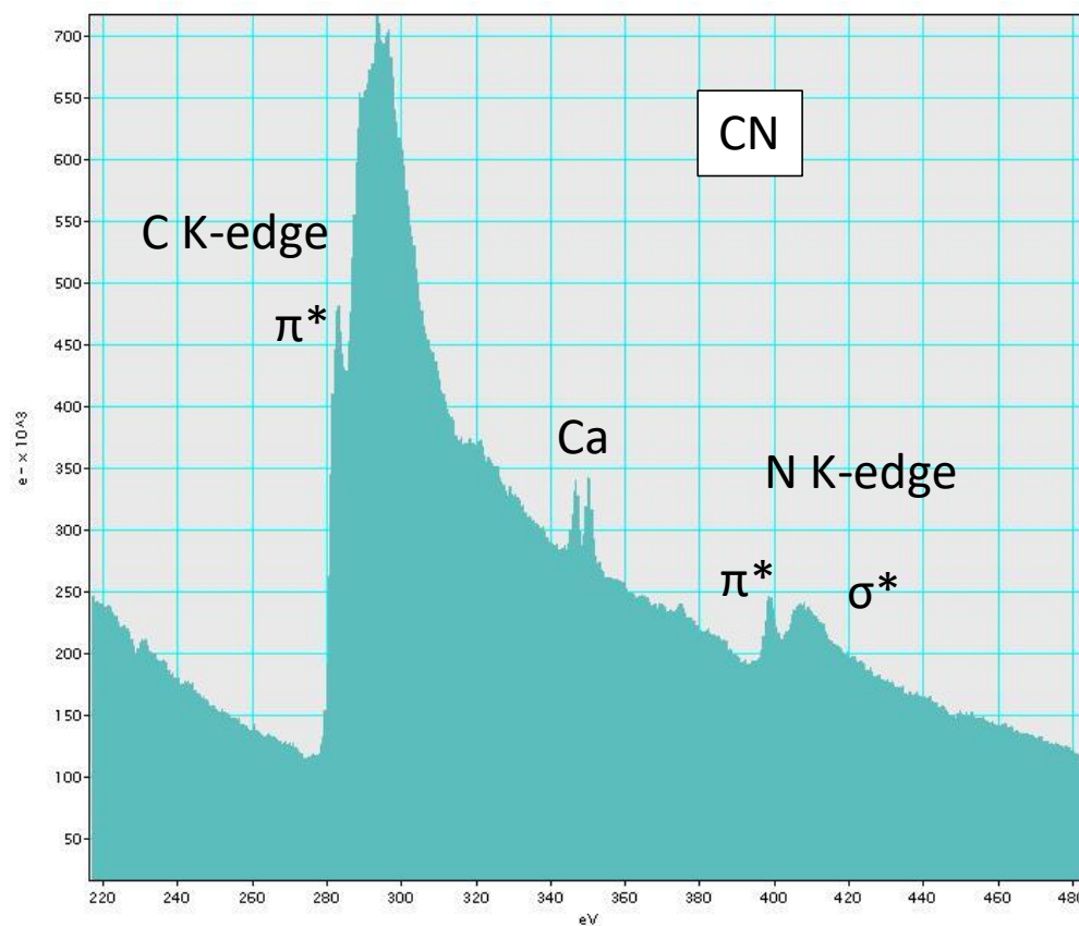
Figure 12. EELS analysis of CN.
