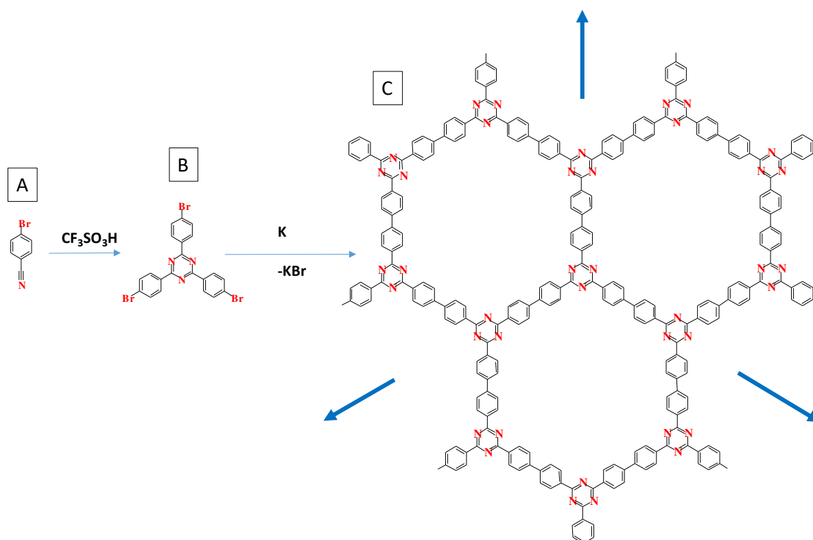
Figure 23 : Synthesis of 2D material by reduction of a polyhalogenated triazine derivative.
