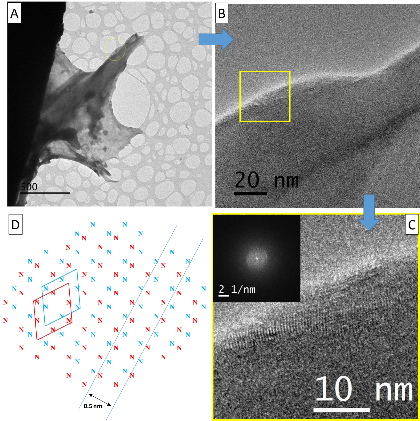
Figure 21 : TEM analysis of a C 2 N flake showing a moiré effect. A) the observed flake; B) zoom over the yellow circle figure A; C) zoom over the yellow square Figure B (insert: FFT of the image); D) two stacked C 2 N layers (blue and red, only nitrogen atoms shown for clarity, unit cells shown as rhombus) exhibiting the observed 0.5 nm distance.
