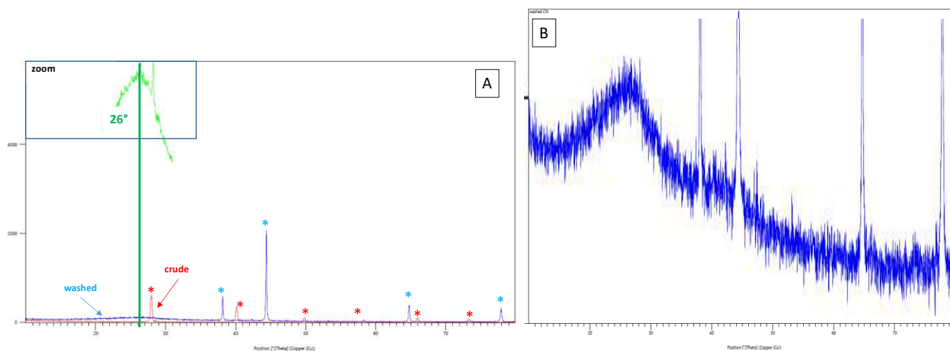
Figure 9 : A) compared powder X-ray diffractograms of a crude (red) and washed (blue) CN samples (same batch). Insert (green): zoom over the blue curve. B) Powder X-ray diffractogram of a washed CN sample Blue stars : signals from the aluminum sample holder ; red stars : signals from KCl by-product.
