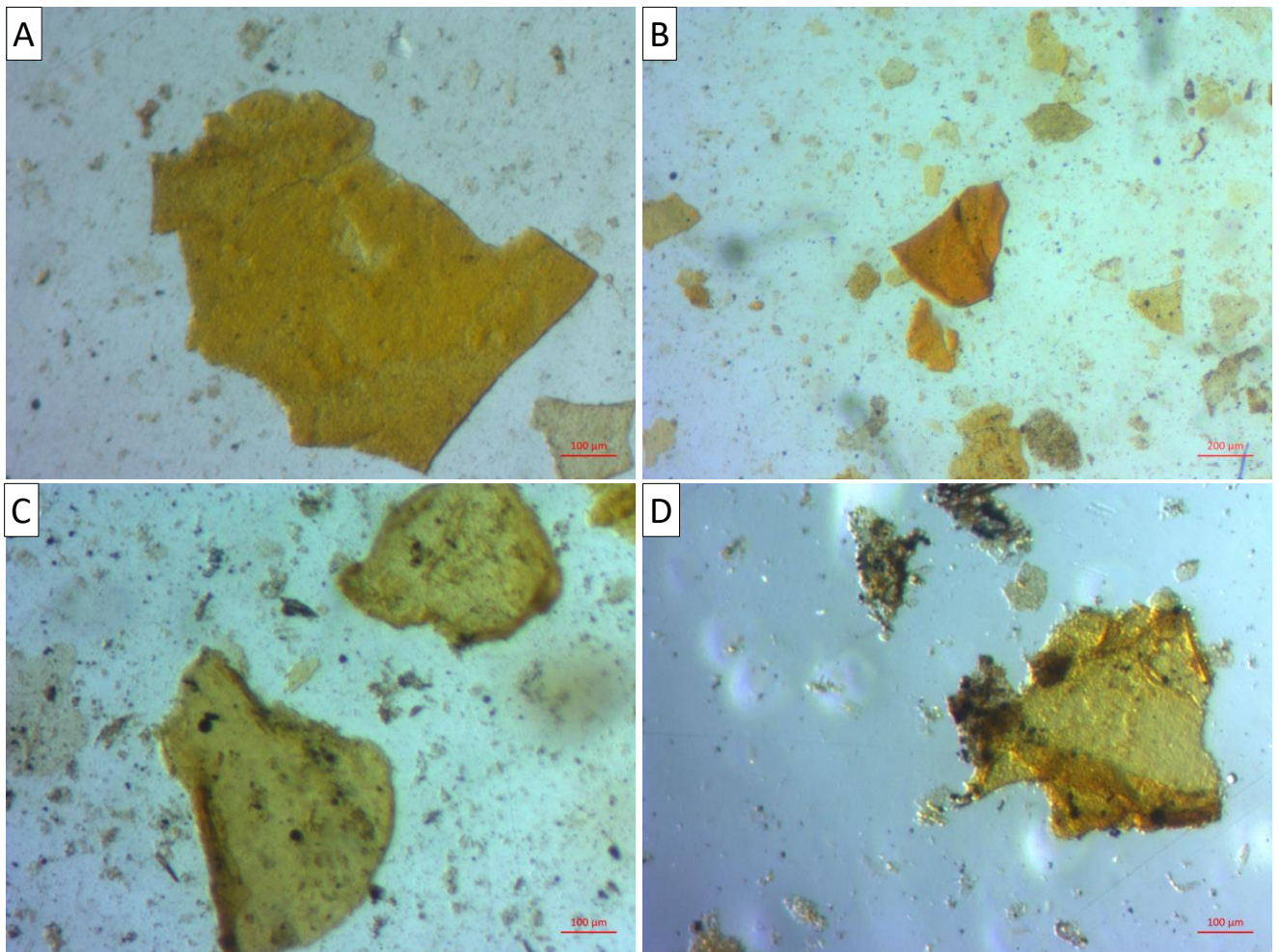
Figure 31: optical microscopy analysis of C_2N obtained using Hg/K amalgam. The flakes were suspended in a 1 : 2 / EtOH : HCl 2M (v/v) solution.
