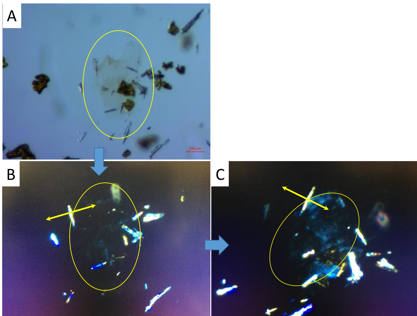
Figure 25: polarised light study of a thin CTF 2D flake (yellow circle). A): normal light; B): the same flake under cross polarized light and C) same sample upon rotation (yellow arrows on B and C as a guide to the eye). The appearance of the flake alternatively goes brighter and darker as a function of the angle. Bright crystals of the starting product are also observed.
