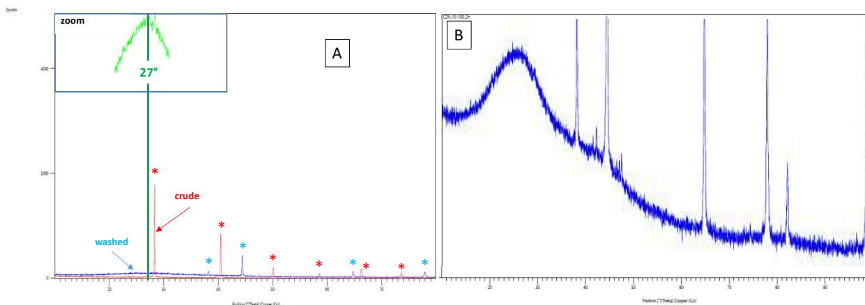
Figure 16 : A) compared powder X-ray diffractograms of a crude (red) and washed (blue) C_2N samples (same batch). Insert (green): zoom over the blue curve. Blue stars : signals from the aluminum sample holder ; red stars : signals from KCl by-product. B) : Powder x-ray diffractogram of the washed C_2N sample. Black stars : signals from the aluminum sample holder.
