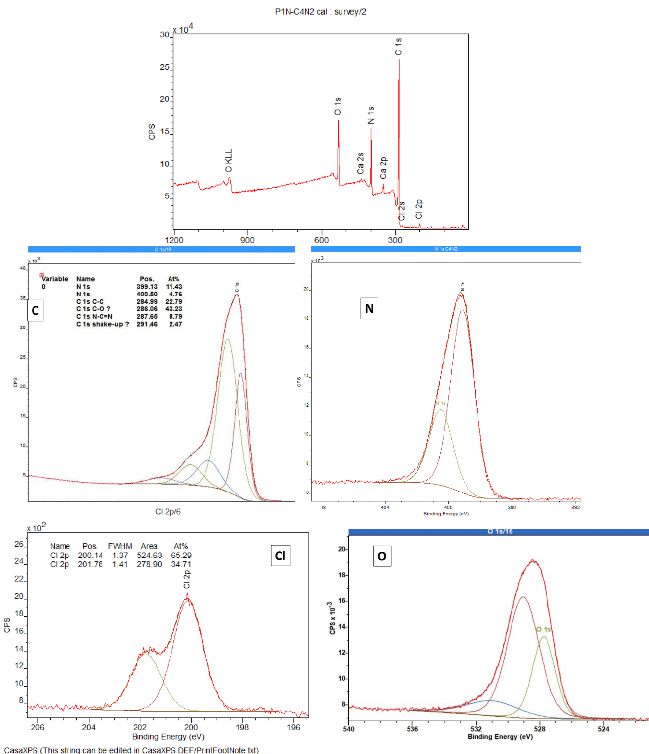
Figure 17 : XPS analysis of a washed C 2 N sample.
