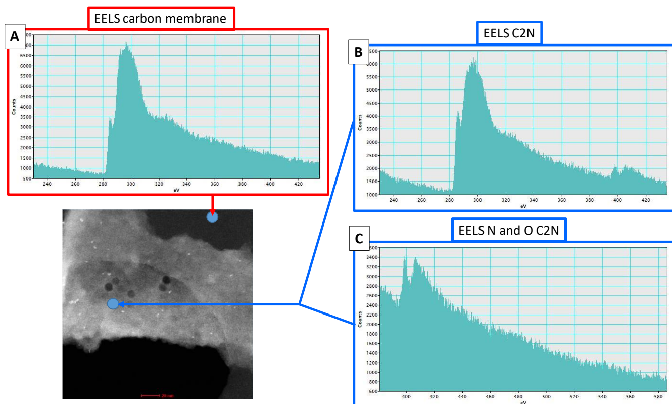
Figure 22 : EELS analysis of a single C 2 N flake suspended on holey carbon grid. A): carbon grid analysis, B) and C): C 2 N sample. The regular, circular holes observed on the sample are due to electron-beam-induced damages.
