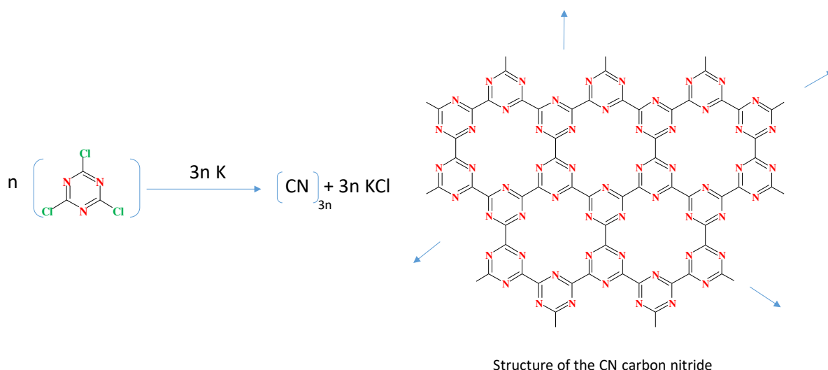
Figure 2: synthesis of CN carbon nitride.
