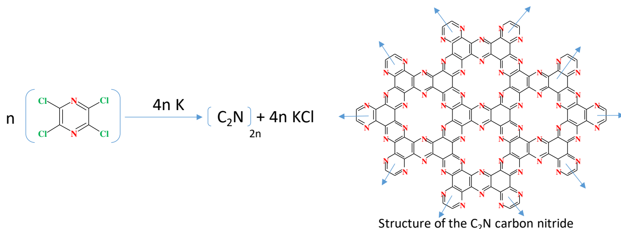
Figure 13. Synthesis of C 2 N.
