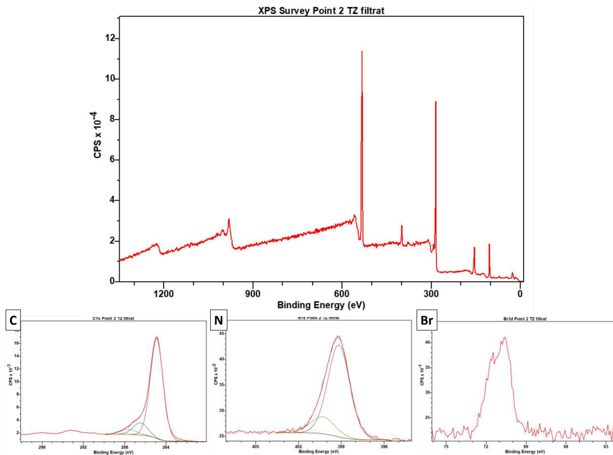
Figure 29 : XPS analysis of CTF-2D material.
