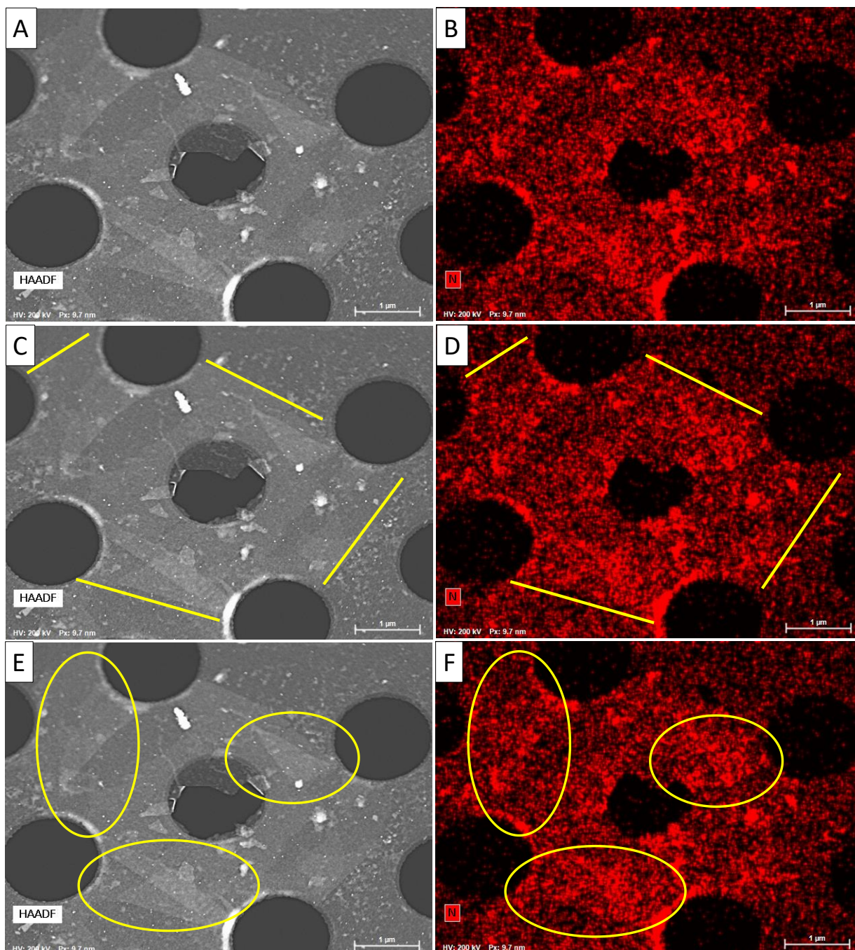
Figure 11. EDS map of CN at the N-K edge.
