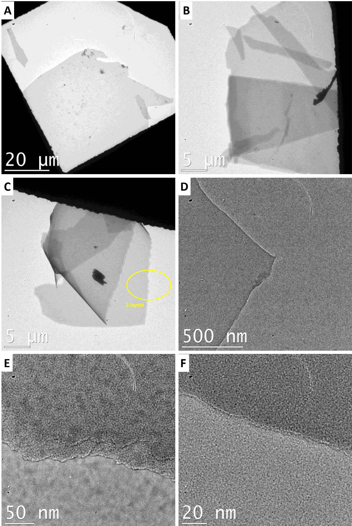
Figure 10. TEM images of CN flakes.
