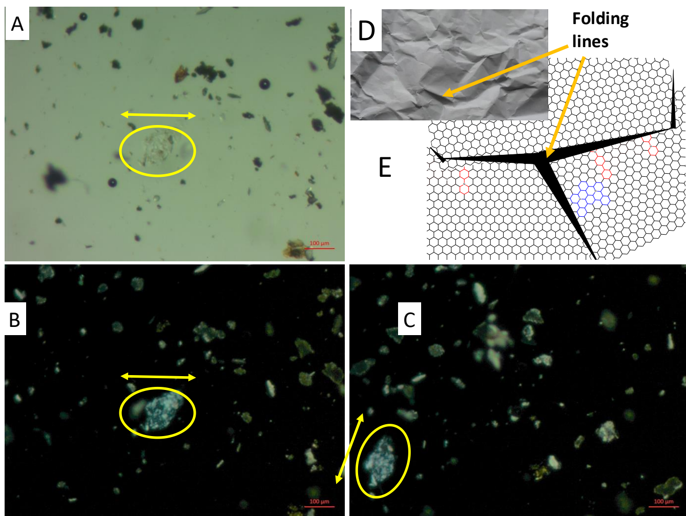
Figure 5: polarized optical microscopy analysis of a CN flake (yellow circle). A) normal light; B) and C) polarised light. The brightness of the flake changes as a function of the angle, evidencing its crystallinity. D) and E): a simple model showing how foldings may give rise to different domains inside a single crystal flake.
