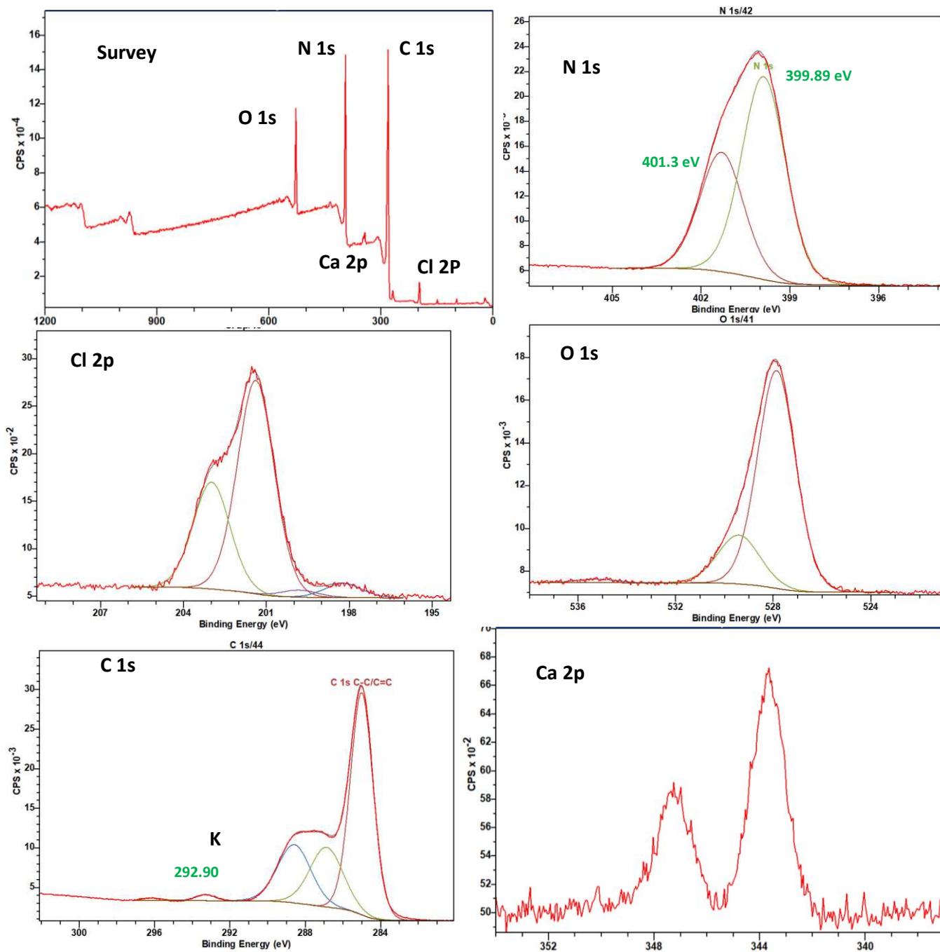
Figure 8. XPS analysis of CN.
