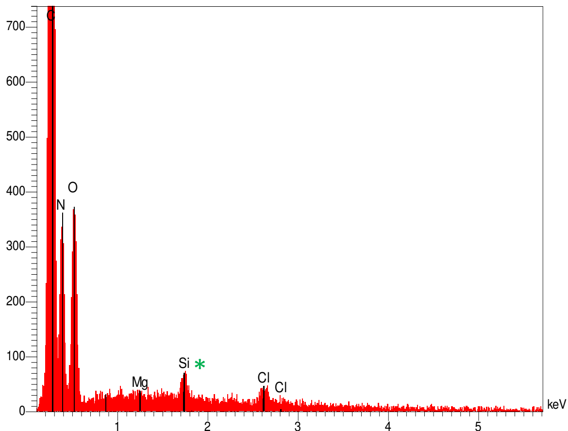
Figure 19: EDS analysis of a washed C 2 N sample (star : signal from the substrate).
