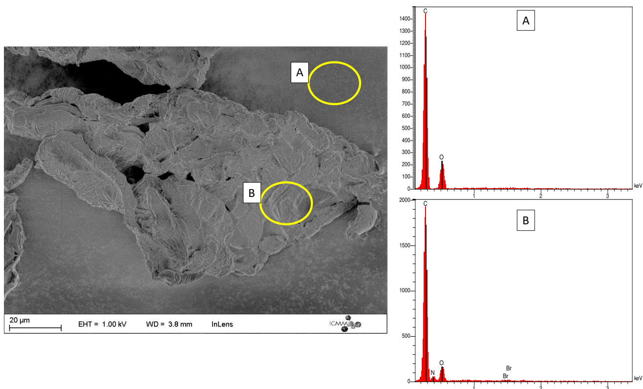
Figure 26: SEMM/EDS analysis of CTF-2D material.
