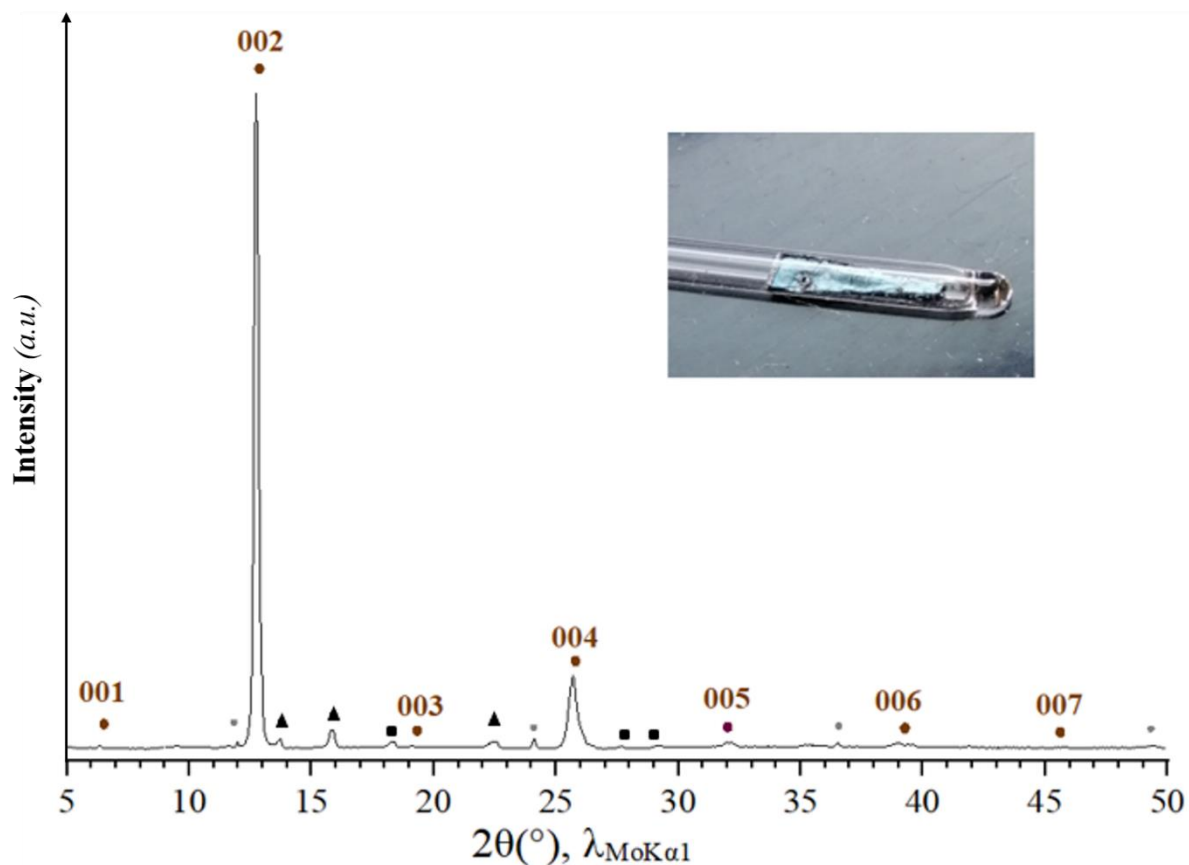
Figure 1: 00 l X-ray diffractogram of the Sr-based GIC and picture of the corresponding sample
