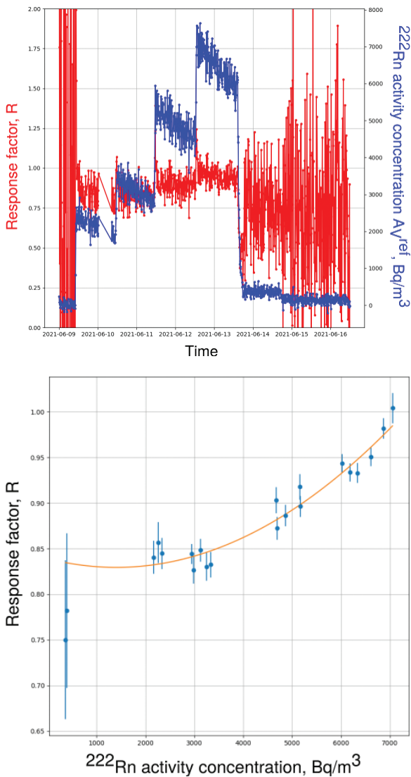
Fig. 6. Left: example of the results of the exposure performed at Sofia University. The blue line indicates A_v^{\text{ref}}(t) , and the red line indicates the observed response factor for one of the instruments. Right: example of the observed non-linearity of the response of REs. The uncertainty bars on the right figure indicate the overall estimated statistical uncertainty of the response factor.
