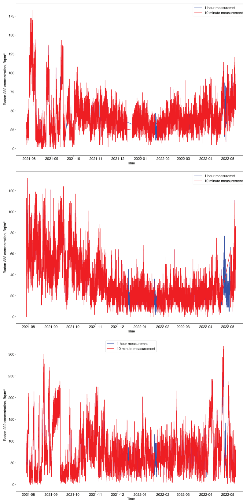
Fig. 10. Data collected from 10-month exposure of RE07-dwelling (top), RE11-workplace (middle) and RE33-dwelling (bottom) detectors. The red line indicates the Web 222 Rn data collected over the Internet (Wi-Fi connection of the instrument to the Web), and the blue line indicates the Bluetooth RE data. The data are used to calculate the quantities shown in Table 4.
