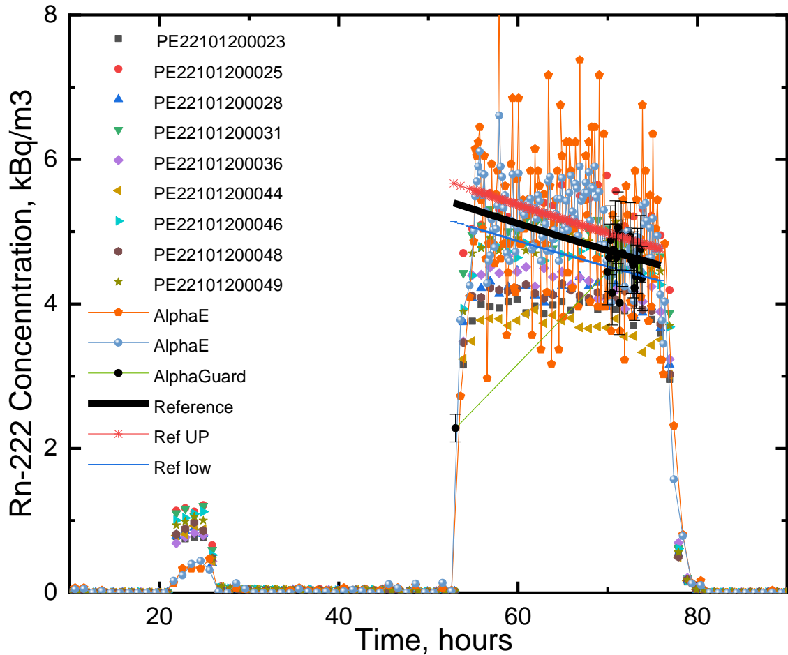
Figure 9. Exposure of the instruments at LNE-LNHB. The black dots show the readings of the Reference instrument. The black solid line (Reference) shows the reference ^{222}\text{Rn} activity concentration ( A_V^{ref}(t) ) during the exposure. The lines “Ref UP” and “Ref low” show the one-sigma interval around the reference activity concentration ( A_V^{ref}(t) \pm \sigma_{A_V^{ref}(t)} ).
