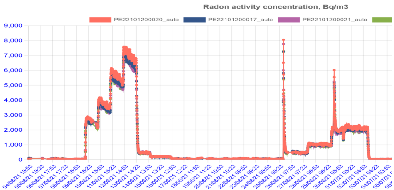
Fig. 4. Examples of two exposures (first: 08/06/21 – 16/06/21; second: 25/06/21 – 03/07/21 ) of ^{222}\text{Rn} measurement instruments at Sofia University. All the readings are from the four RadonEye instruments.
