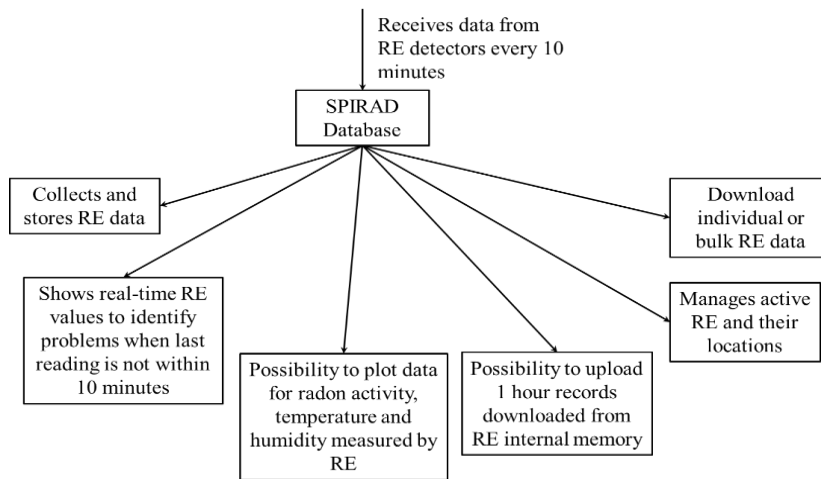
Figure 1. Schematic representation of the SPIRAD database and its functionality.
