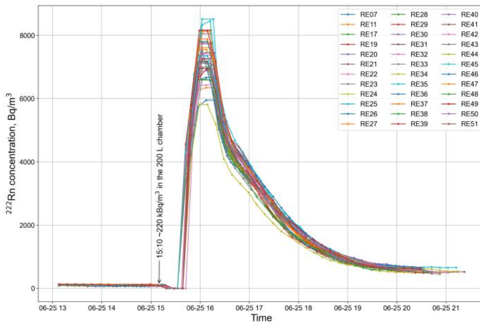
Fig. 8. After high activity spike all detectors record zeroes. Immediately after flushing the exposure chamber with clean air, there is significant difference between the detector readings while they return to their working range. The time format on the abscissa is “Month-day hour”.
