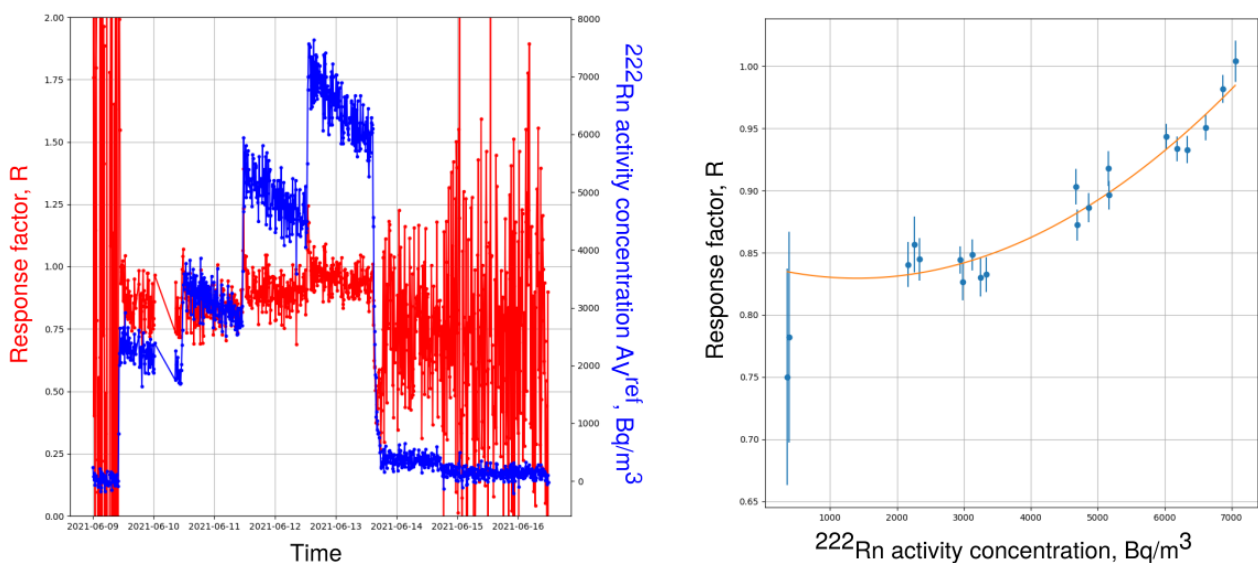
Fig. 6. Left: example of the results of the exposure performed at Sofia University. The blue line indicates A_V^{ref}(t) and the red line indicates the observed response factor for one of the instruments. Right: example of the observed non-linearity of the response of REs. The uncertainty bars on the right figure indicate the overall estimated statistical uncertainty of the response factor.
