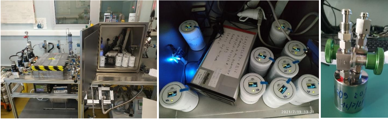
Fig. 5. The ^{222}\text{Rn}/^{220}\text{Rn} laboratory facility at LNHB (left). Center: The REs in the system together with the reference instrument AlphaGUARD. Right: The volume used to transfer the radon in the system from the primary ^{222}\text{Rn} standard.
