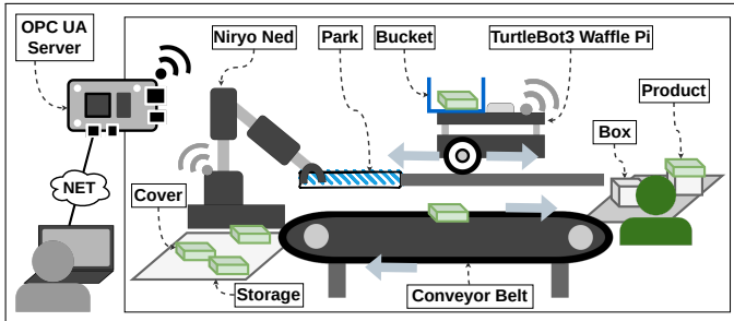
Fig. 5. The architecture of the fault-tolerant PAL case study of LocalSEA
