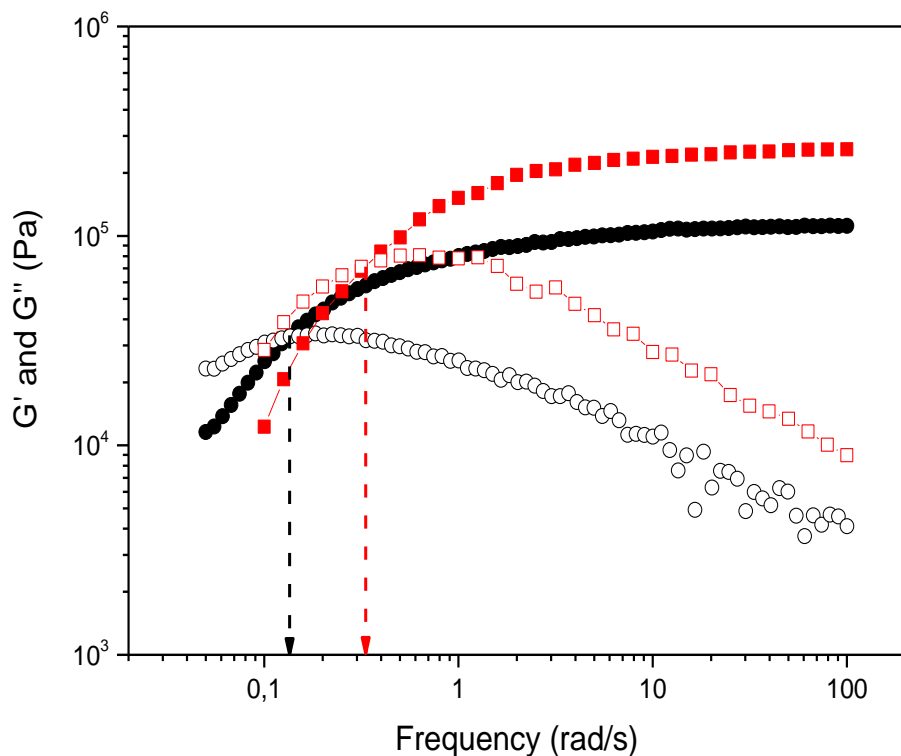
Figure 5 Viscoelasticity of a) mixed phytantriol-10-GMO (3:1 molar ratio) -water cubic gel (black) and b) phytantriol cubic gel (red) at 30% water. Full symbol for G' and empty symbol for G'' .
