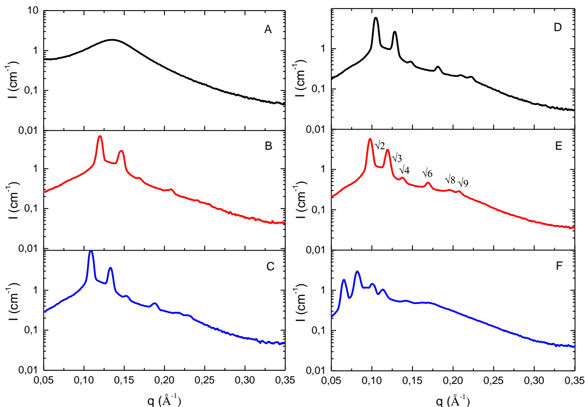
Figure 3 Scattering profiles of ternary phyantriol-10-GMO mixtures (3:1) as a function of (A) 10%wt, (B) 15%wt, (C) 20%wt, (D) 25%wt, (E) 30%wt, and (F) 50%wt water content.
