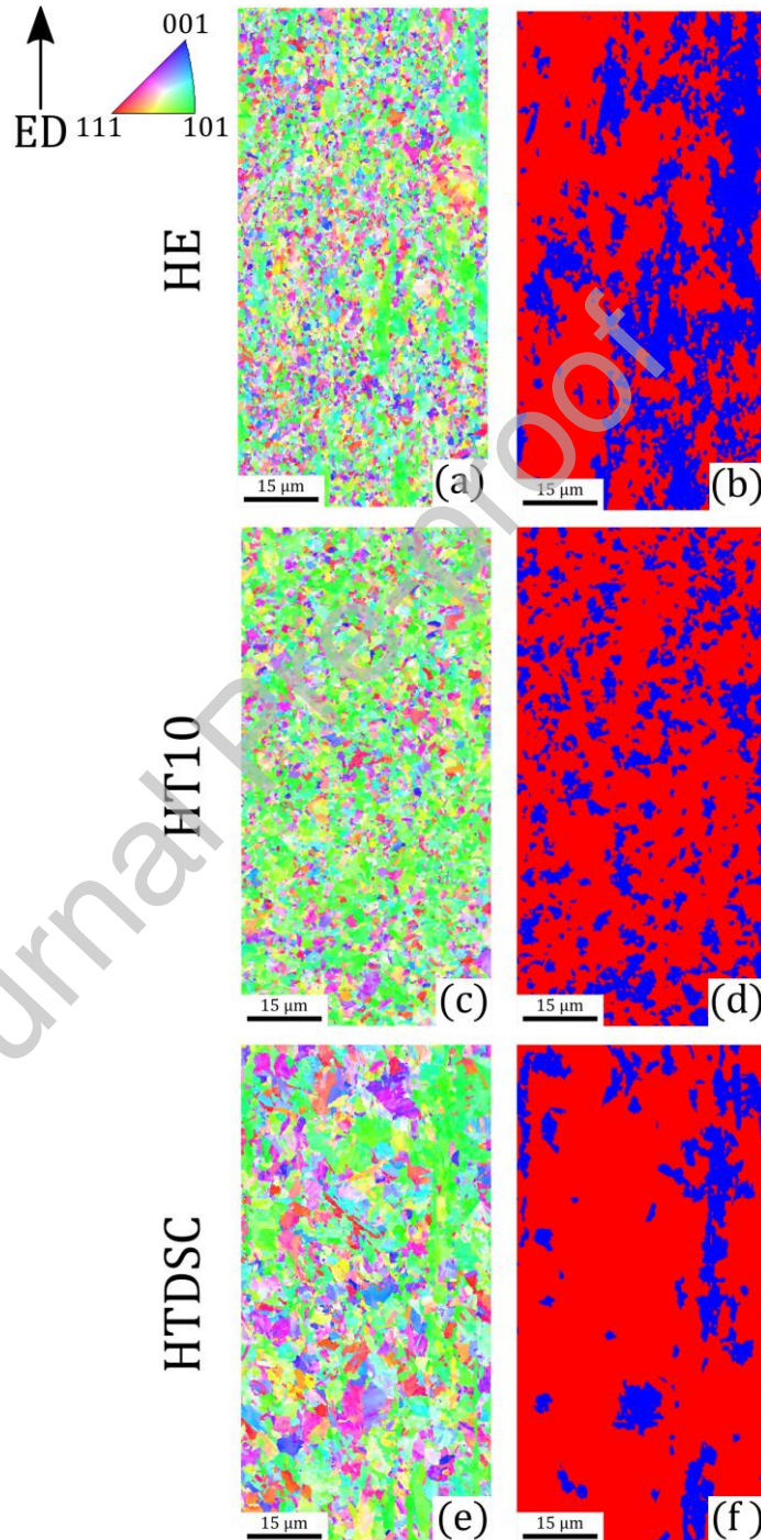
Figure 6 : Inverse pole figure map \langle uvw \rangle direction parallel to the extrusion direction ED of (a) HE quenched, (c) HT10 quenched and (e) HTDSC quenched. IQ threshold map of (b) HE quenched, (d) HT10 quenched and (f) HTDSC quenched, martensite area are in red and UF area are in blue.
