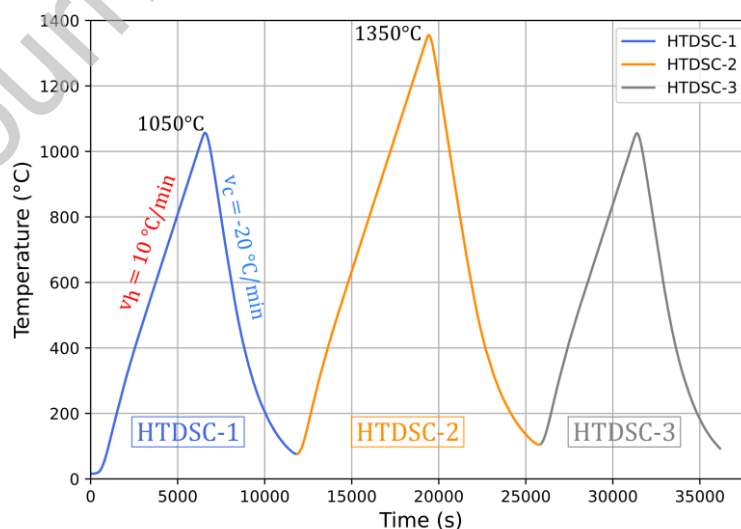
Figure 1 : Heat treatments of HTDSC sample. The first cycle in blue is HTDSC-1 (1050°C), the second in orange is HTDSC-2 (1350°C) and the third in grey is HTDSC-3 (1050°C).
