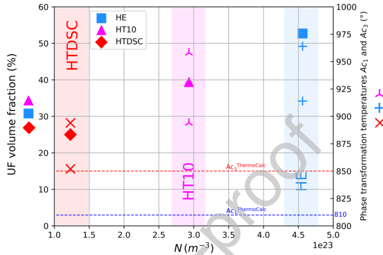
Figure 7 : UF volume fraction measured by DSC and phase transformation temperatures Ac_1 , Ac_3 measured by DSC with a heating rate of 10°C/min as a function of the nano-oxides density obtained by SAXS with Monte Carlo method. The dot lines represent Ac_1 and Ac_3 obtained from ThermoCalc calculations for to the 10Cr materials of the study without the oxide dispersion contribution [14].
