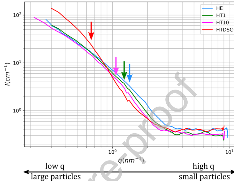
Figure 5 : Scattering curves of HE, HT1, HT10 and HTDSC samples. Arrows indicate the q -position of the main particles contribution on scattering.
