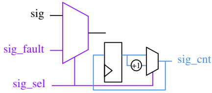
Fig. 2: Logical representation of a fault controller for signal sig added in the SMT model of the CPU.
