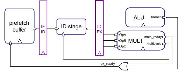
Fig. 4: Multiplier input/output signals and their use to stall the preceding pipeline stages in case of multicyle multiplication.
