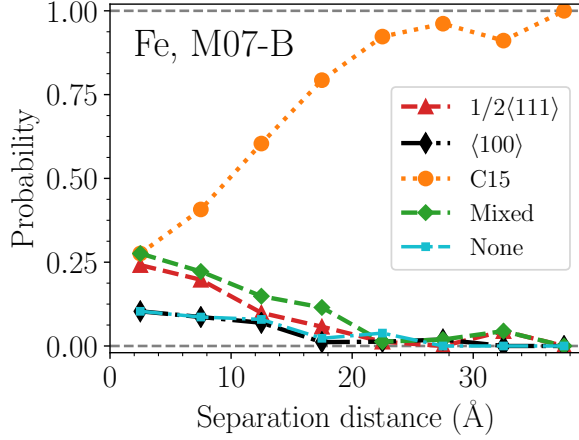
Figure 14: Observed probabilities of forming different types of SIA clusters as functions of separation distance, for 5 keV cascades on a pre-existing 40 SIA C15 cluster at 300 K in the M07-B potential.
