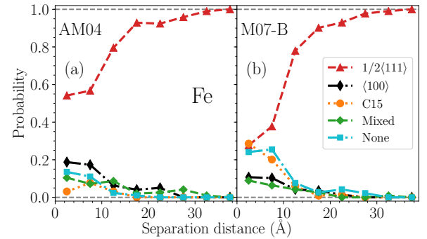
Figure 11: Example of the observed probabilities of forming different types of SIA clusters as functions of separation distance in Fe. The data is from 3 keV cascades overlapping with a 30 SIA 1/2\langle 111 \rangle loop at 300 K, for both the AM04 and M07-B potentials.
