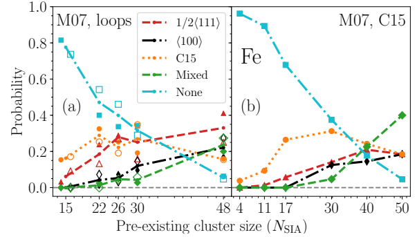
Figure 16: Observed probabilities of forming different types of SIA clusters at full overlap, for 5 keV cascades at 300 K in the M07 potential. In figure (a), the pre-existing clusters are dislocation loops (filled points for pre-existing 1/2\langle 111 \rangle loops and unfilled points for \langle 100 \rangle loops). In figure (b), the pre-existing clusters are C15 clusters.
