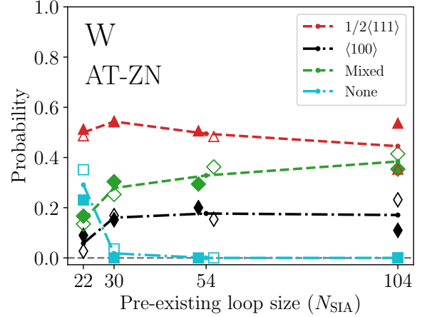
Figure 19: Observed probabilities of forming different types of SIA clusters at full overlap, for 10 keV cascades at 300 K in the AT-ZN potential. For filled data points, the pre-existing cluster was a 1/2\langle 111 \rangle loop, and for unfilled data points a \langle 100 \rangle loop. The lines connect the average values of both pre-existing loop types.
