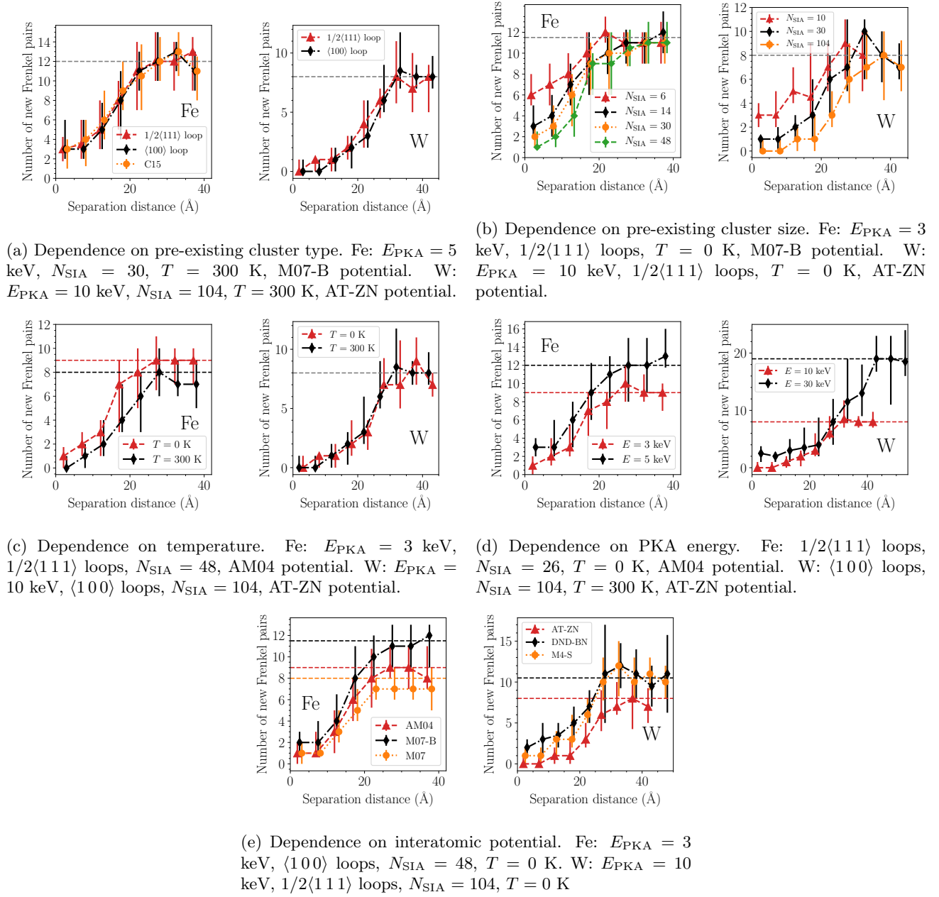
Figure 2: Examples of the reduced defect production for cascades overlapping with SIA clusters in iron and tungsten, as functions of separation distance (i.e the centre-to-centre distance between the pre-existing cluster and the disordered cascade region). Simulation details are given below each figure. Each data point is the median value in a bin containing in the order of 50–100 simulations. The horizontal lines show the median number of Frenkel pairs in cascades in the defect-free material. The error bars show the interquartile range, i.e. the spread of the data around the median. The data points are slightly shifted in the x axis direction to make the error bars visible.
