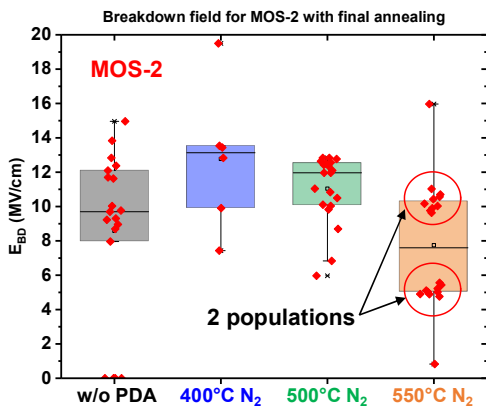
Fig. 6: Breakdown field obtained from I-V measurements of MOS-2 devices after the final thermal budget. 550°C has a degradation of E_{BV} with two populations.
