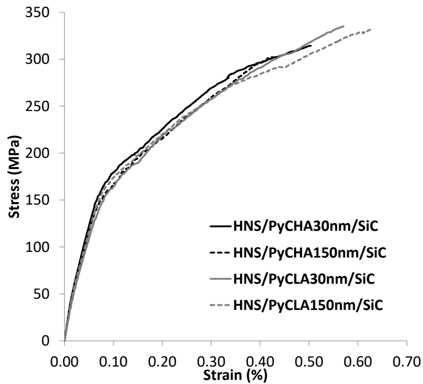
Figure 7. Influence of PyC texture and thickness on the tensile stress–strain behavior.
