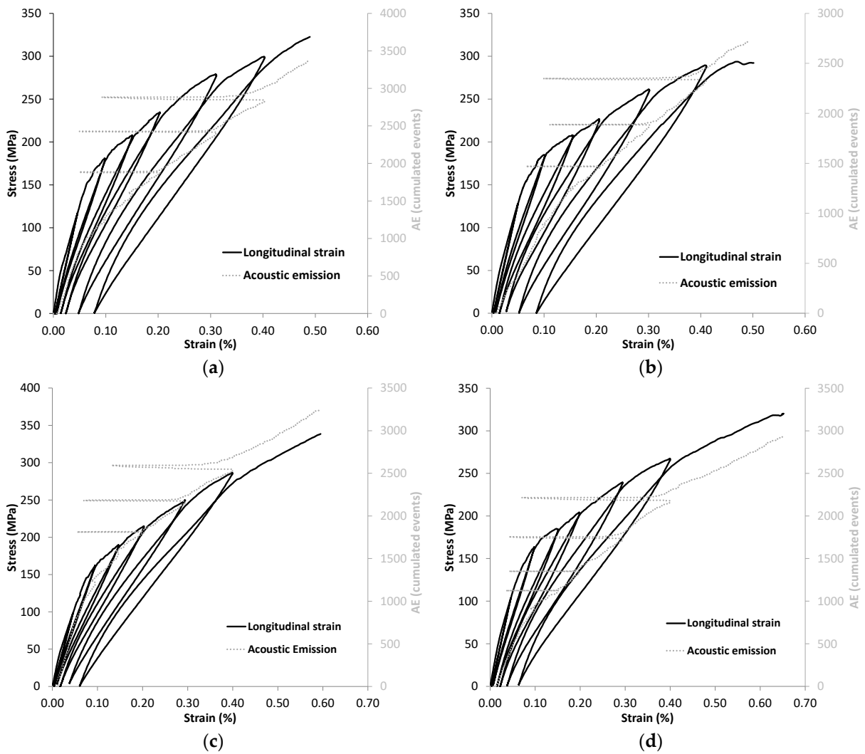
Figure 9. Typical tensile stress–strain behaviors with unloading–reloading sequences with evolution of cumulated AE signal for (a) HNS/PyC HA30nm /SiC, (b) HNS/PyC HA150nm /SiC, (c) HNS/PyC LA30nm /SiC and (d) HNS/PyC LA150nm /SiC.
