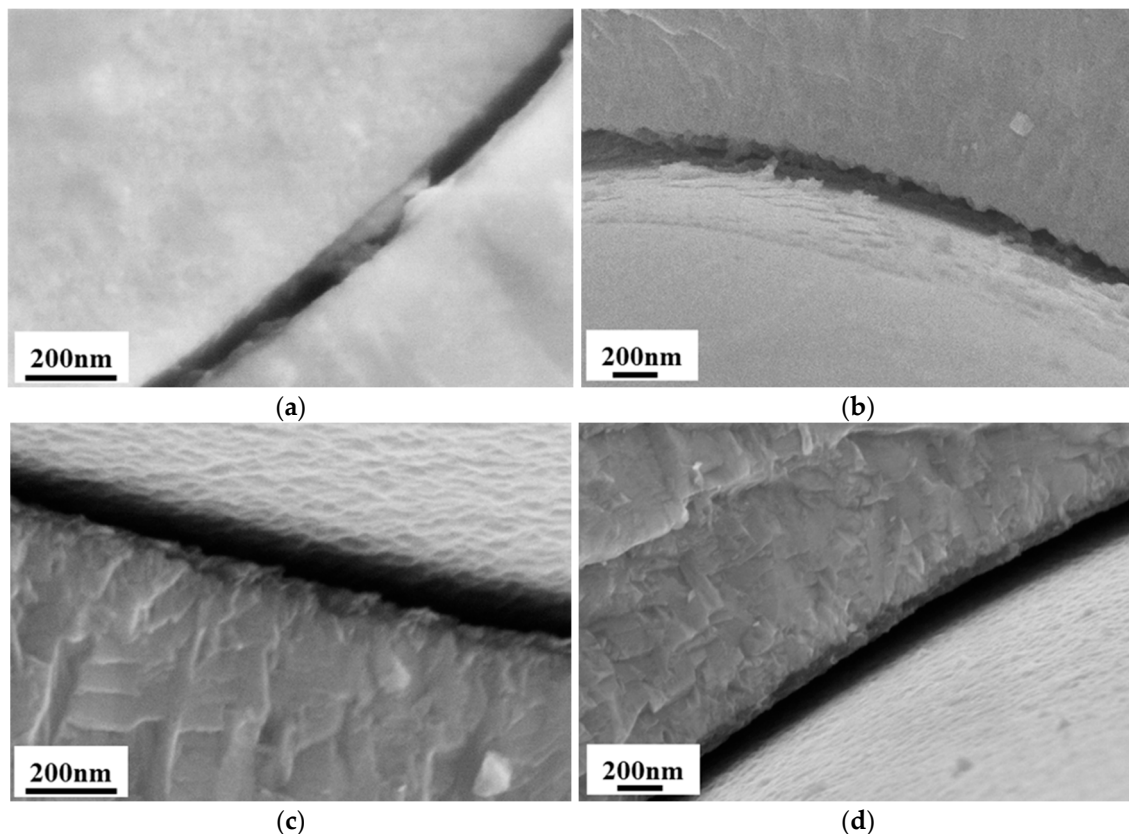
Figure 11. High magnification SEM micrographs of typical F/M debonding zone after failure for each type of composites specimen: (a) HNS/ \text{PyC}_{\text{HA}30\text{nm}} /SiC, (b) HNS/ \text{PyC}_{\text{HA}150\text{nm}} /SiC, (c) HNS/ \text{PyC}_{\text{LA}30\text{nm}} /SiC and (d) HNS/ \text{PyC}_{\text{LA}150\text{nm}} /SiC.
