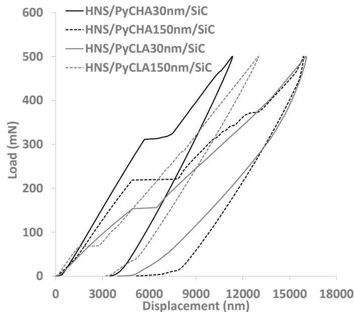
Figure 5. Typical push-out test curve of HNS/ \text{PyC}_{\text{HA}30\text{nm}}/\text{SiC} , HNS/ \text{PyC}_{\text{HA}150\text{nm}}/\text{SiC} , HNS/ \text{PyC}_{\text{LA}30\text{nm}}/\text{SiC} and HNS/ \text{PyC}_{\text{LA}150\text{nm}}/\text{SiC} .
