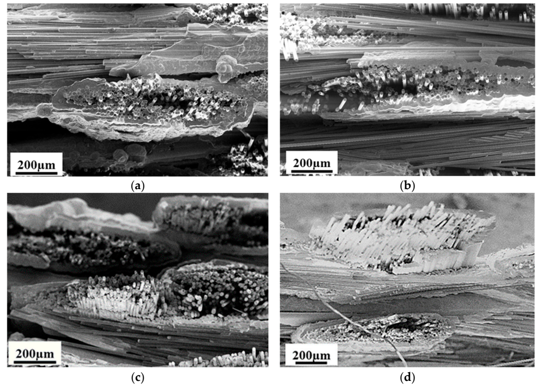
Figure 8. Fracture surface after failure for each type of composites specimen: (a) HNS/PyC HA30nm /SiC, (b) HNS/PyC HA150nm /SiC, (c) HNS/PyC LA30nm /SiC and (d) HNS/PyC LA150nm /SiC.
