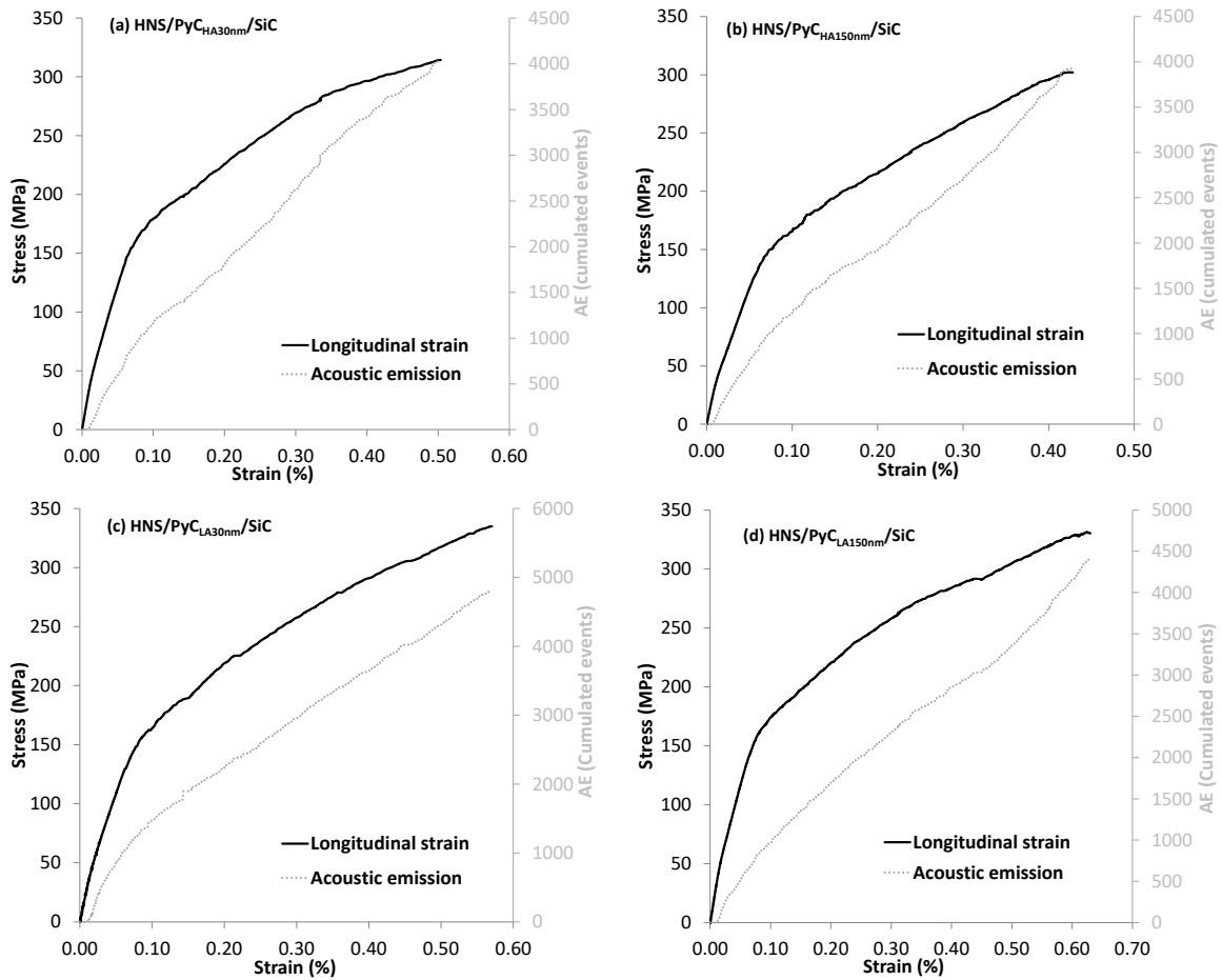
Figure 6. Typical tensile stress–strain curves.
