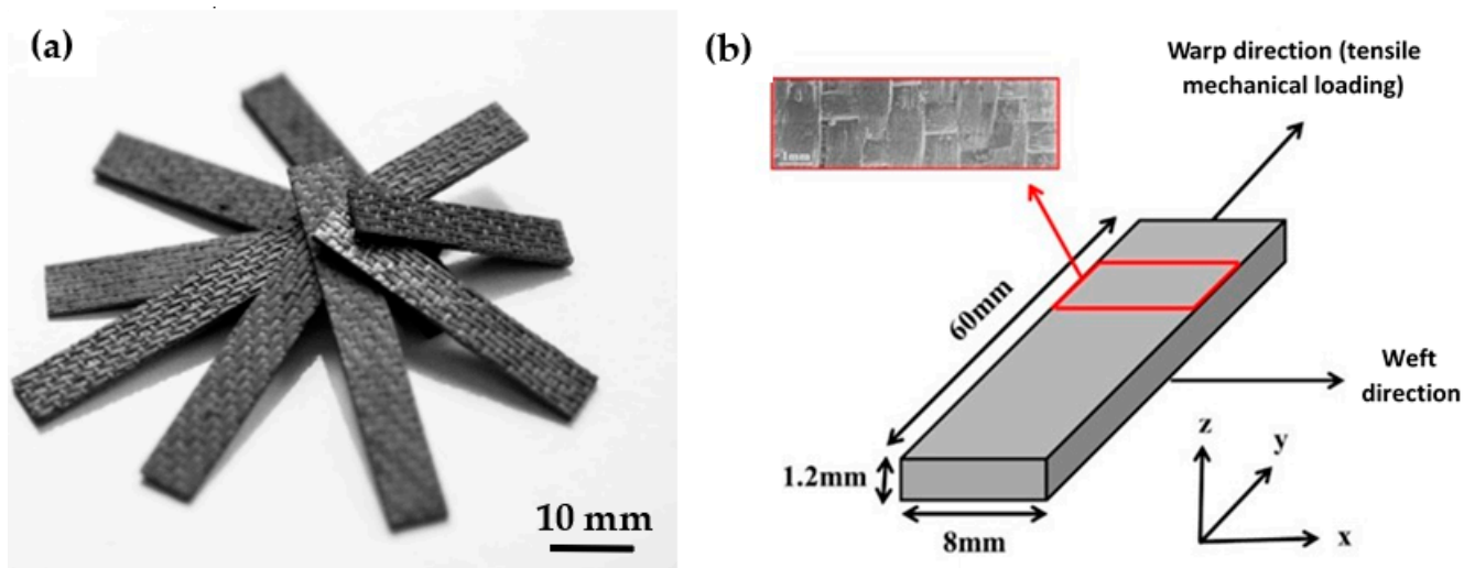
Figure 1. SiC/SiC composites specimens as processed: (a) global picture and (b) specimen orientations for tensile mechanical tests.
