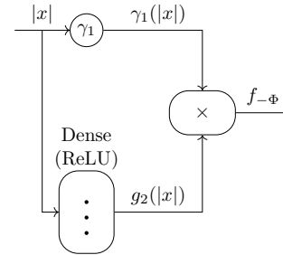
(b) Predistorsion function for AM/PM distortion
