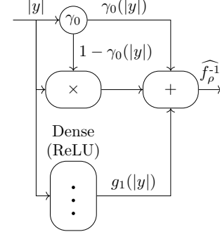
(a) Predistorsion function for AM/AM distortion
