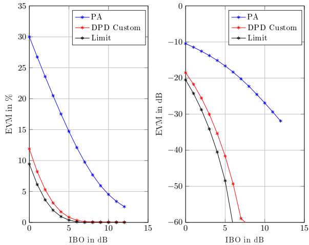
Fig. 6. EVM performance in [dB] using “conventional” learning
