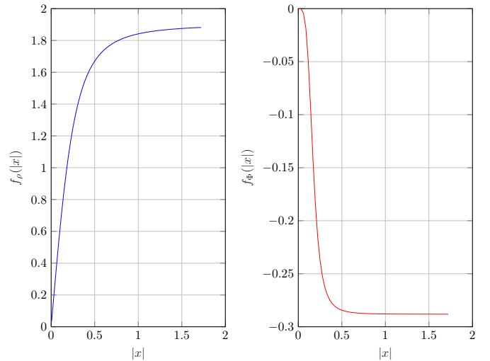
Fig. 5. AM/AM and AM/PM characteristics of Rapp PA [8]
