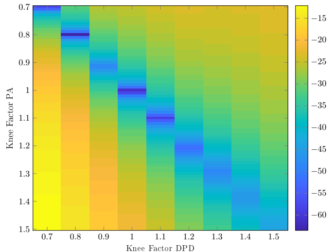
Fig. 3. EVM performance in [dB] with 0.7 \leq p \leq 1.5
