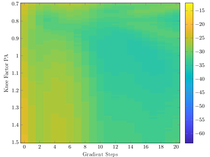
Fig. 7. EVM performance in [dB] with 0.7 \leq p \leq 1.5
