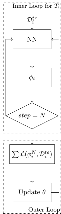
Fig. 4. MAML algorithm
