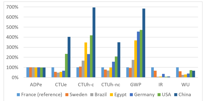
Fig. 5. Comparison of LCA results of the transmitter antenna over its life cycle depending on use stage location.
