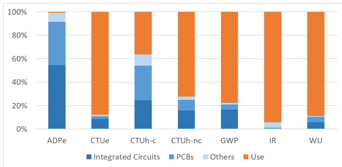
Fig. 3. LCA results of the transmitter antenna. 100% represents the complete life cycle (manufacturing + use). “Others” category is composed of connectors, solders, resistors and capacitors.
