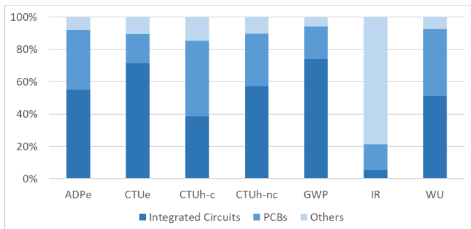
Fig. 4. LCA results of the transmitter antenna. 100% represents the complete manufacturing stage. “Others” category is composed of connectors, solders, resistors and capacitors.
