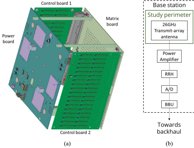
Fig. 1. (a) Studied transmitarray antenna. (b) The system perimeter represents a small part of a base station. RRH: Remote Radio Head, A/D: Analog-Digital converter, BBU: Base Band Unit.
