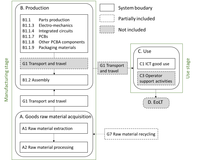
Fig. 2. System boundaries according to ITU L.1410 standard [15].
