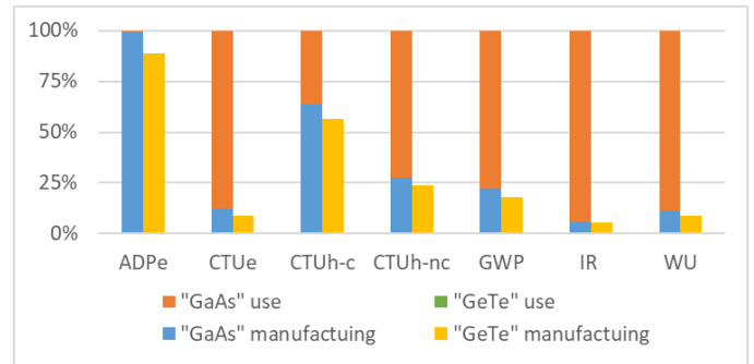
Fig. 6. Comparison between the GaAs diode technology and the GeTe switch technology over the antenna life cycle for a specific backhaul application case.
