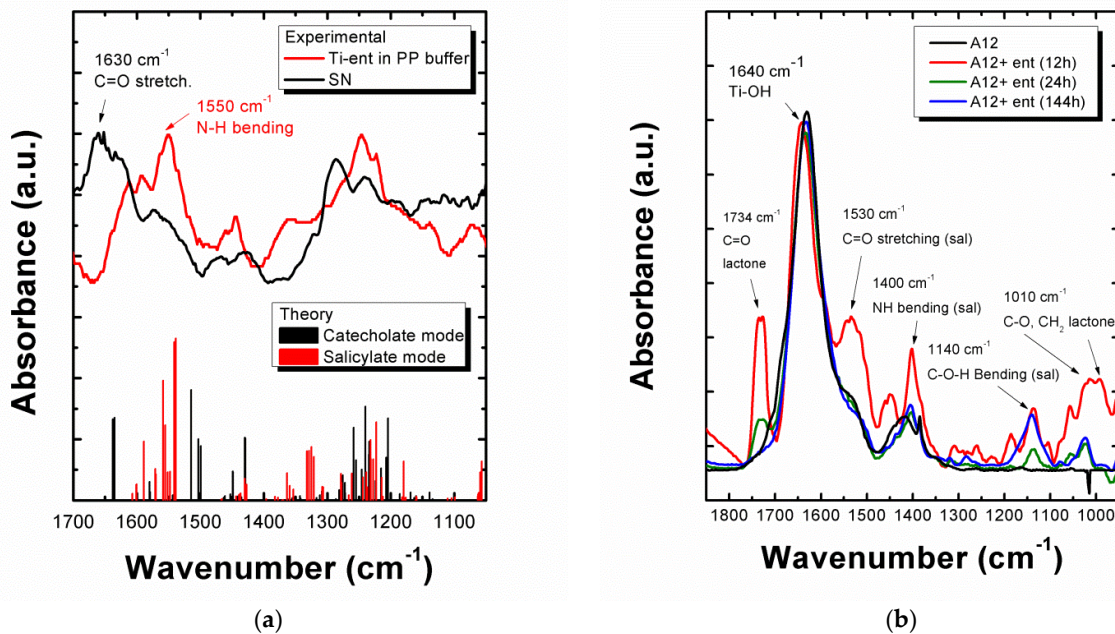
Figure 4. (a) FTIR spectra of the SN collected after 24 h of incubation at 37 ^{\circ}\text{C} of \text{TiO}_2 -A12 (5 mg/mL) in the presence of enterobactin ( \text{ent} ) (100 \mu\text{M} ) in PP buffer compared to the spectra of a solution of \text{Ti-ent} complex (100 \mu\text{M} in PP medium). The peaks were assigned according to theoretical calculations of \text{Ti-ent} complexes in salicylate and catechol mode (see Supplementary Materials, Section A). (b) FTIR spectra of the powders obtained after incubation of \text{TiO}_2 -A12 with \text{ent} (50 \mu\text{M} ) at different incubation times. The spectra were normalized from the \text{TiO}_2 -specific peak at 1640 \text{cm}^{-1} ( \nu\text{Ti-OH} ).
