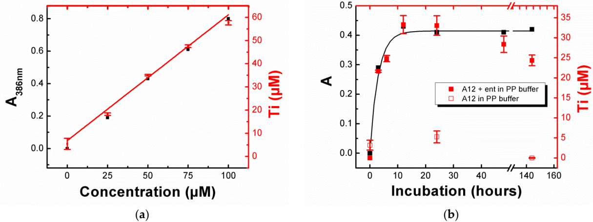
Figure 3. The influence of \text{ent} concentration and incubation time on the solubilization of \text{TiO}_2 -A12 NPs (5 mg/mL) in PP medium. UV-visible absorbance at 386 nm (black) and Ti quantified by ICP-AES (red) as a function of (a) \text{ent} concentration after 24 h incubation, and (b) incubation time with \text{ent} (50 \mu\text{M} ). Error bars were determined by calculating the standard deviation of duplicate experiments. Red squares correspond to A12 incubation in the PP buffer in the presence (filled square) or absence of \text{ent} (open square).
