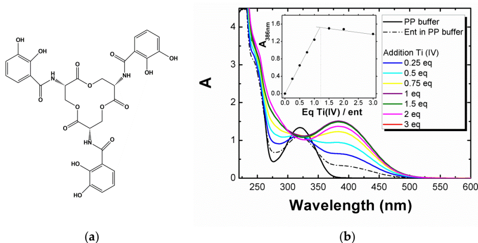
Figure 1. (a) Molecular structure of the enterobactin siderophore (ent) and (b) enterobactin metallation (100 \mu M) followed by UV–visible spectroscopy by successive additions of Ti(IV) equivalent (TiCl 4 , 1 mM) in the PP medium. (Inserts) Determination of the stoichiometry of the Ti–enterobactin complex by following the evolution of the absorbance at 386 nm during addition of Ti(IV). A = absorbance.
