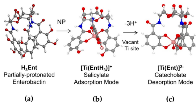
Figure 6. Surface solubilization mechanism of the TiO 2 -NPs by enterobactin. The mechanism consists of (a) the approach of a partially protonated enterobactin near neutral pH toward the TiO 2 NP surface; (b) the binding to a Ti site in the salicylate mode via one or two bidentate catechols group(s) first, and then its full chelation; and (c) the rate-limiting detachment of the Ti atom, leading to the release of a catecholate Ti-ent complex (1:1 stoichiometry) in the environment, followed by a proton-exchange reaction with the vacant site to regenerate the surface.
