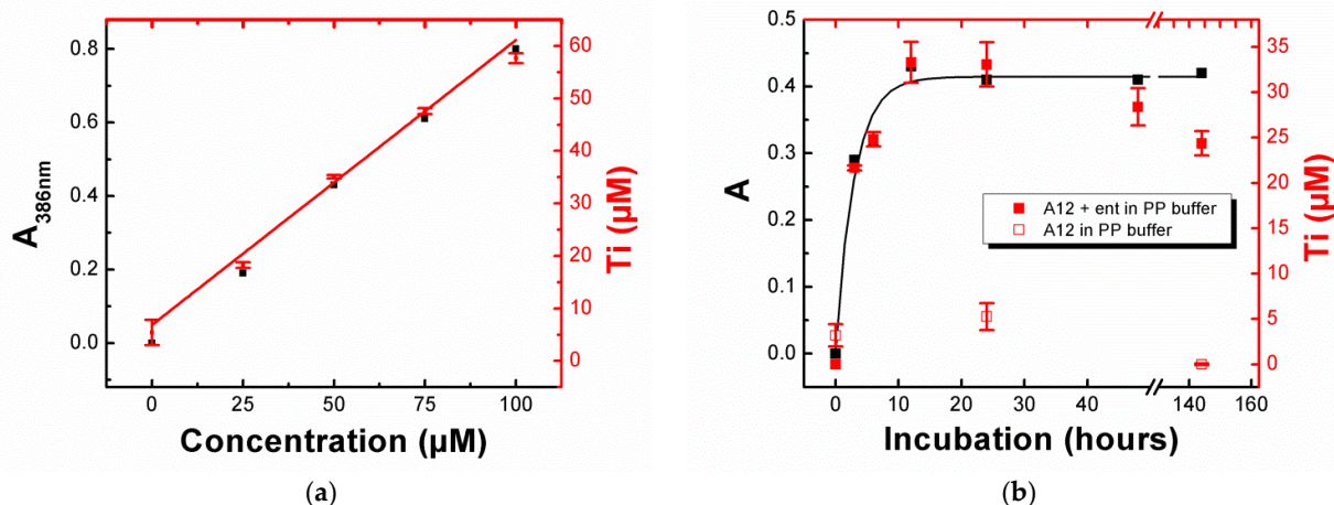
Figure 3. The influence of ent concentration and incubation time on the solubilization of TiO_2 -A12 NPs (5 mg/mL) in PP medium. UV-visible absorbance at 386 nm (black) and Ti quantified by ICP-AES (red) as a function of (a) ent concentration after 24 h incubation, and (b) incubation time with ent (50 \mu M ). Error bars were determined by calculating the standard deviation of duplicate experiments. Red squares correspond to A12 incubation in the PP buffer in the presence (filled square) or absence of ent (open square).
