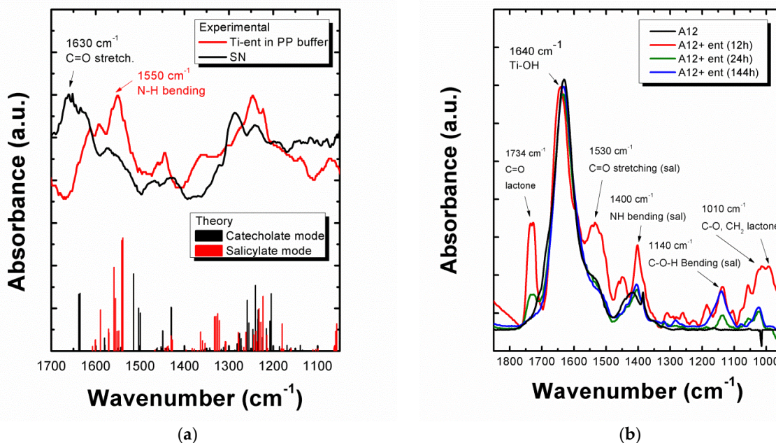
Figure 4. (a) FTIR spectra of the SN collected after 24 h of incubation at 37 ^{\circ}C of TiO_2 -A12 (5 mg.mL ^{-1} ) in the presence of enterobactin ( ent ) (100 \mu M ) in PP buffer compared to the spectra of a solution of Ti- ent complex (100 \mu M in PP medium). The peaks were assigned according to theoretical calculations of Ti- ent complexes in salicylate and catechol mode (see Supplementary Materials, Section A). (b) FTIR spectra of the powders obtained after incubation of TiO_2 -A12 with ent (50 \mu M ) at different incubation times. The spectra were normalized from the TiO_2 -specific peak at 1640 cm^{-1} ( \nu Ti-OH ).
