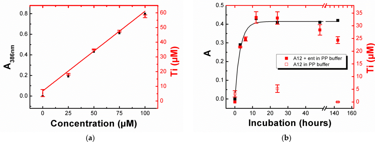
Figure 3. The influence of \text{ent} concentration and incubation time on the solubilization of \text{TiO}_2 -A12 NPs (5 mg/mL) in PP medium. UV-visible absorbance at 386 nm (black) and Ti quantified by ICP-AES (red) as a function of (a) \text{ent} concentration after 24 h incubation, and (b) incubation time with \text{ent} (50 \mu\text{M} ). Error bars were determined by calculating the standard deviation of duplicate experiments. Red squares correspond to A12 incubation in the PP buffer in the presence (filled square) or absence of \text{ent} (open square).
