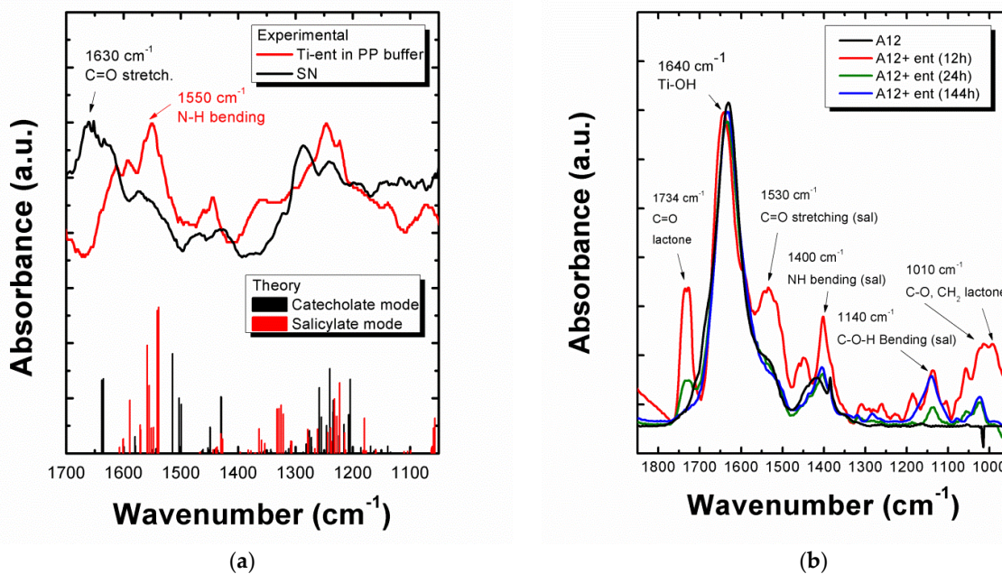
Figure 4. (a) FTIR spectra of the SN collected after 24 h of incubation at 37 °C of \text{TiO}_2 -A12 (5 mg/mL) in the presence of enterobactin ( \text{ent} ) (100 \mu\text{M} ) in PP buffer compared to the spectra of a solution of \text{Ti-ent} complex (100 \mu\text{M} in PP medium). The peaks were assigned according to theoretical calculations of \text{Ti-ent} complexes in salicylate and catechol mode (see Supplementary Materials, Section A). (b) FTIR spectra of the powders obtained after incubation of \text{TiO}_2 -A12 with \text{ent} (50 \mu\text{M} ) at different incubation times. The spectra were normalized from the \text{TiO}_2 -specific peak at 1640 \text{cm}^{-1} ( \nu\text{Ti-OH} ).
