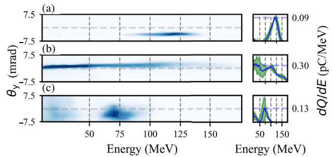
FIG. 6. Same as Fig. 5 for laser focus at z = 0 mm with three consecutive shots included in the standard deviation.
