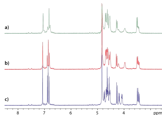
Fig. 3 ^1\text{H} NMR spectrum of a mixture of cryptophanes 1 and 2 in \text{D}_2\text{O} ( B_0 = 11.7 T; T = 298 K). a) as is; b) after having degassed the solution; c) after addition of ca. 5 mM of xenon. Concentration of 1 = 51 \mu\text{M} ; concentration of 2 = 49 \mu\text{M} . Small signals visible on spectra a-c are characteristic of the 'non-canonical' forms of compound 1 (see text).
