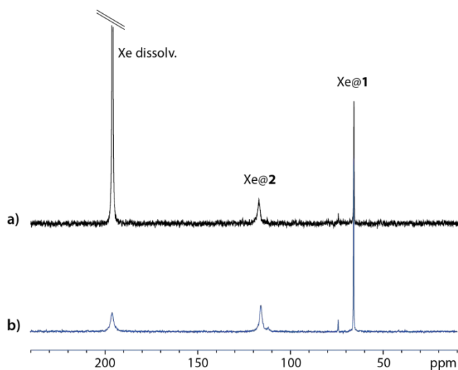
Fig. 2 One-scan ^{129}\text{Xe} NMR spectra obtained on a mixture of compounds 1 (0.51 mM) and 2 (0.49 mM) in \text{D}_2\text{O} + \varepsilon NaOD, at a) high xenon concentration, b) low xenon concentration (sum of three experiments). B_0 = 11.7 T; T = 298 K.
