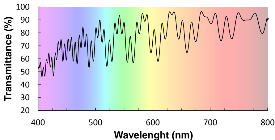
Fig. 3. Transmittance spectrum of ITO/PZT/ITO/SiO 2 membrane in the 400-800 nm range.
