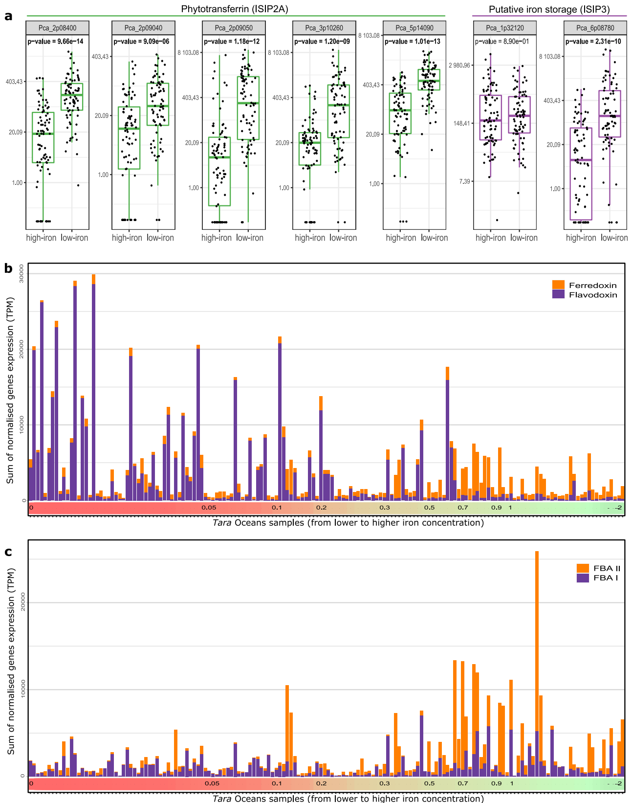
Fig. 4 Expression of iron-related genes in P. calceolata . a Relative gene expression levels normalized in transcript per million (TPM) of five phytotransferrins (ISIP2A) and two putative iron storage (ISIP3) in low-iron (<0.2 nM) and high-iron (>0.2 nM) oceanic stations. P values of Wilcoxon statistical tests between low- and high-iron conditions are indicated for each gene. Significant P values (<0.01) are in bold. b Relative expression levels (TPM) of genes coding for ferredoxin (orange) and its non-ferrous equivalent flavodoxin (purple) in each Tara Oceans sample. Samples are sorted from low-iron (left) to high-iron (right) conditions. Iron concentrations are indicated in nM on the colored horizontal bar. c Same representation for genes coding for fructose-bisphosphate aldolase II (orange) and its non-ferrous equivalent fructose-bisphosphate aldolase I (purple).
