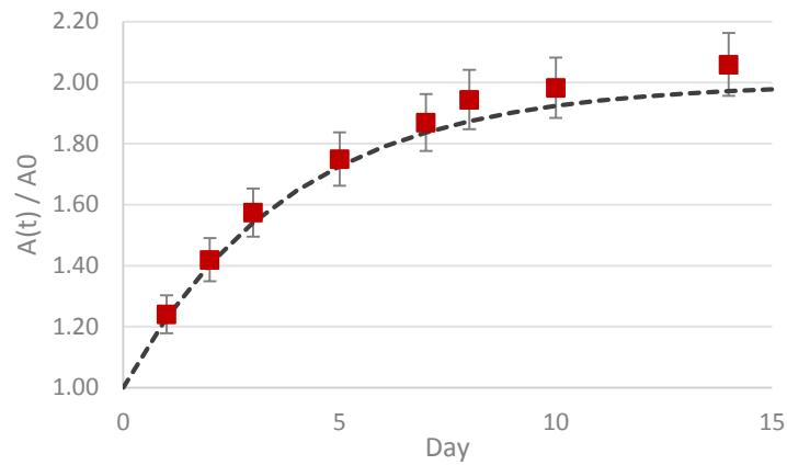
Figure 1: Y-90 growth curve from Sr-90 obtained with plastic scintillation resin selective towards Sr
