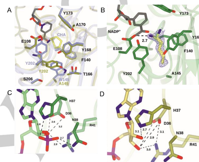
Figure 4. (A) Active sites of CfusAmdH /NADP + complex with cyclohexylamine (CHA, 6IAU, carbon atoms in blue) and CfusAmdH -W145A/NADP + (carbon atoms in gold), showing rotation of Y202 side chain to fill space vacated by W145A mutation; (B) Active site of CfusAmdH -W145A/NADP + complex with pentan-1-amine ( 2a ), modeled in two conformations, each at 50% occupancy. (C) Cofactor binding pocket of CfusAmdH -W145A/NADP + complex (D) Cofactor binding pocket of CfusAmdH -W145A/NAD + . The ionic interaction between D36 and R41 side chains in the NAD + complex is absent in the NADP + complex. Electron density corresponds to the F_o - F_c (omit) map at a level of 3\sigma obtained prior to building and refinement of the ligand. Interaction between the ligand nitrogen atom and E108 side chain is shown as a black dashed line with the distance in Å.
