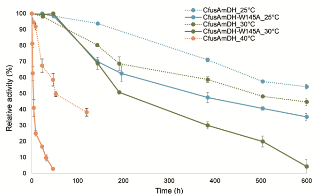
Figure 3. Thermostability of CfusAmdH and CfusAmdH -W145A at 25, 30 and 40 °C. The remaining specific activities were measured as described in the Experimental Section with 0.05 - 0.12 mg mL -1 of purified enzyme, 30 °C. The maximum activity of CfusAmdH towards 1a was 219.2 mU mg -1 and the maximum activity of CfusAmdH -W145A towards 1c was 256.3 mU mg -1 . Error bars represent standard deviations of two or three independent experiments.
