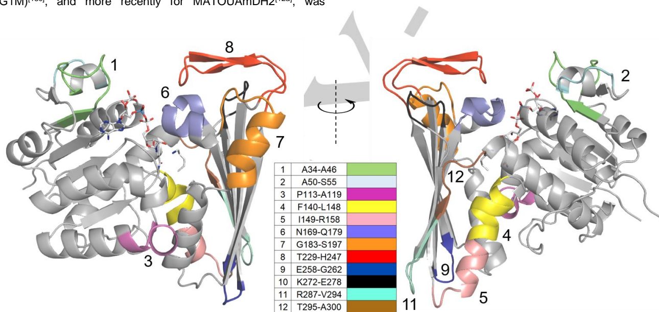
Figure 5. 3D representation at 0° and 180° of WT monomer in complex with NAD and PEN. Segments 1-12, displaying a backbone fluctuation beyond 1.5 Å in Root Mean Square Fluctuation (RMSF) analysis (Figure S18), are highlighted with a gradient of colors reported in the inserted table.
