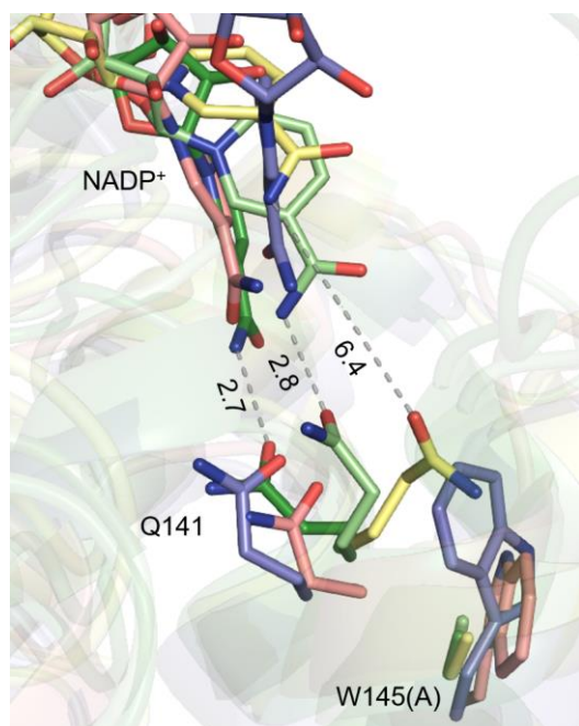
Figure 6. Close-view of Q141 in WT and M at different time of the dynamic. M_NAD_HEP_2 frames at 0.1, 16.2 and 18.5 ns are represented in dark green, light green and yellow, respectively. WT_NAD_HEP_4 at 29.0 ns and WT_NAD_HEP_1 at 53.2 ns are represented in purple and pink, respectively.
