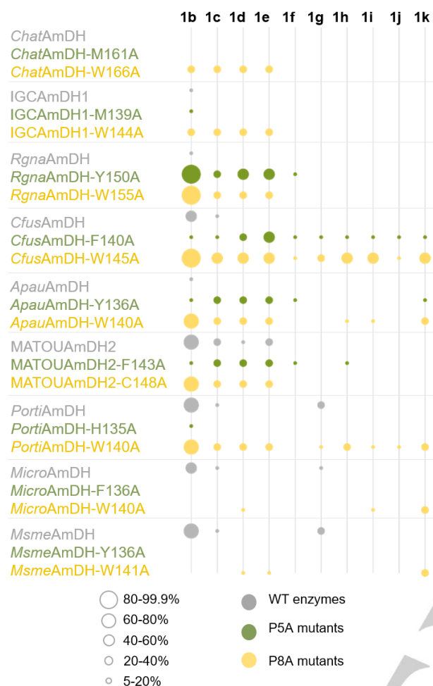
Figure 2. Conversions obtained for WT enzymes and mutants towards substrates 1b - 1k . Reaction conditions: final volume 100 \mu L, 10 mM substrate (DMSO 5% (v/v)), 2 M \text{NH}_4\text{HCO}_2 buffer, pH 8.5, 0.4 mM NAD(P) + , 1.2 eq. D-glucose, 3 U \text{mL}^{-1} GDH-105, 0.5 mg \text{mL}^{-1} purified enzyme, 25 ^\circ\text{C} , 24 h. The monitoring of the remaining aldehydes or ketones 1b-1j , the amines 2b-2j and the corresponding alcohols formed was performed by GC-FID after ethyl acetate extraction. The monitoring of the amine 2k formed was carried out by UHPLC-UV after derivatization with Marfey's reagent (FDAA) (Table S3-S5).
