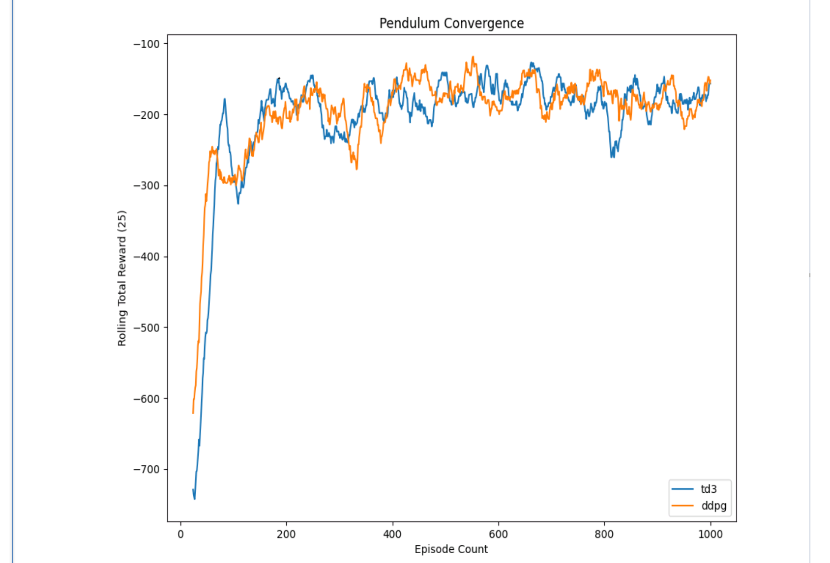
Figure 21. Performance of DDPG versus TD3.
