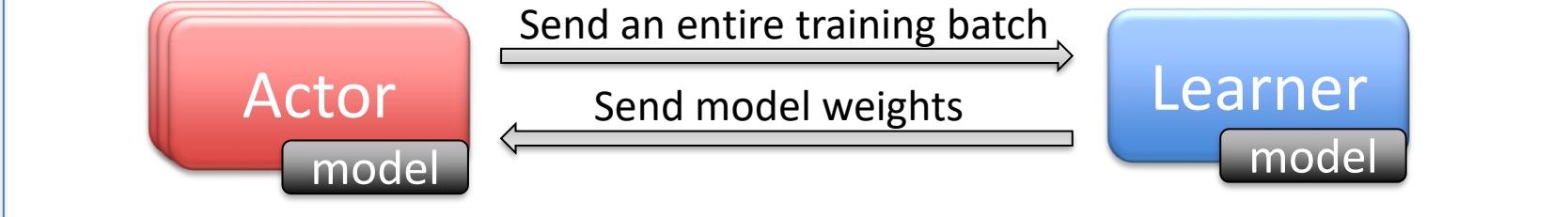
Figure 9. Current EXARL architecture (inspired from IMPALA)
