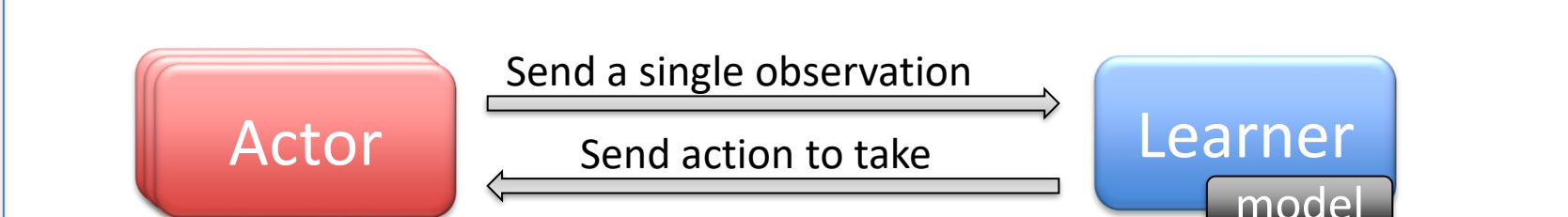
Figure 10. Architecture inspired from SEED (implemented using MPI)
