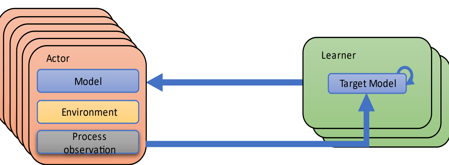
Figure 2. EXARL architecture.
