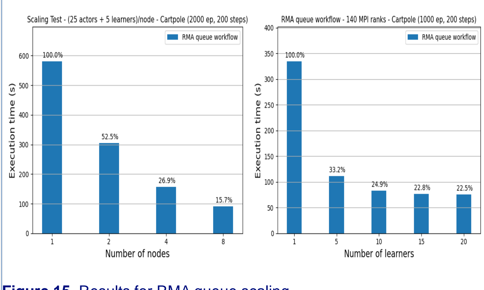
Figure 15. Results for RMA queue scaling
