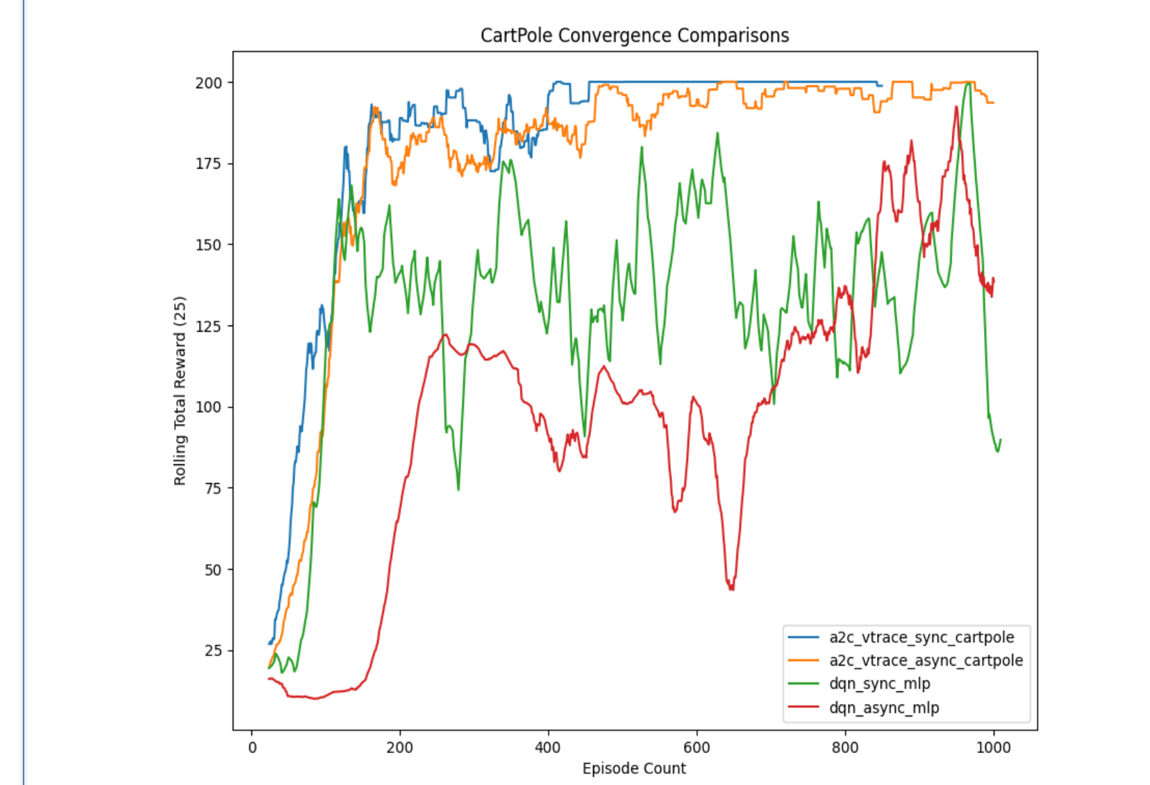
Figure 19. Performance of A2C/A3C versus DQN for CartPole environment. Note that DQN does not converge, whilst A2C/A3C with v-trace does.
