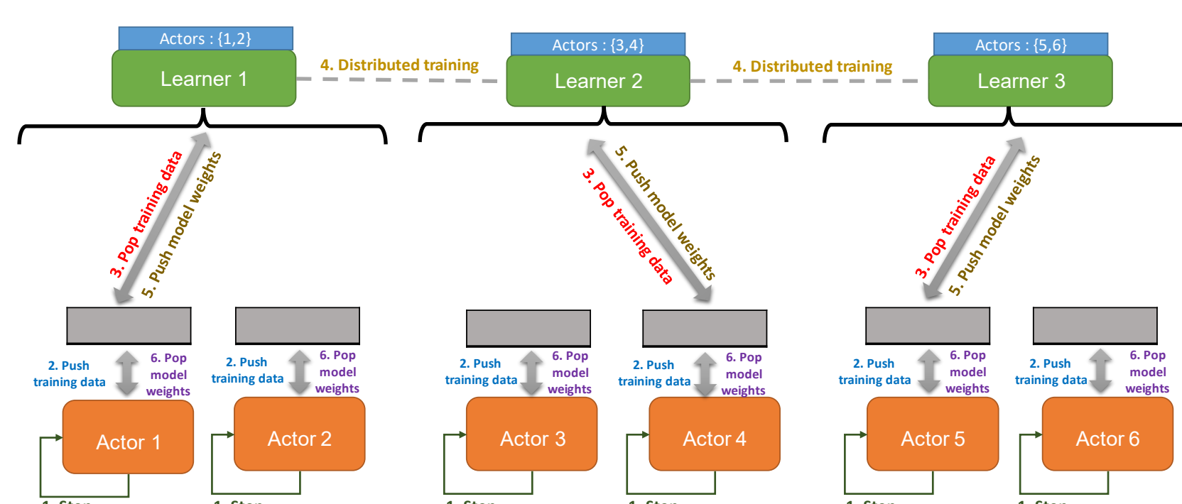
Figure 5. Multi-learner RMA workflow - range-based window selection.
