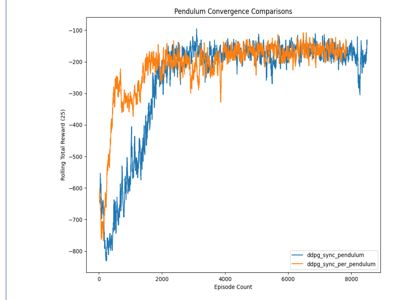
Figure 22. Performance of DDPG with and without PER.
