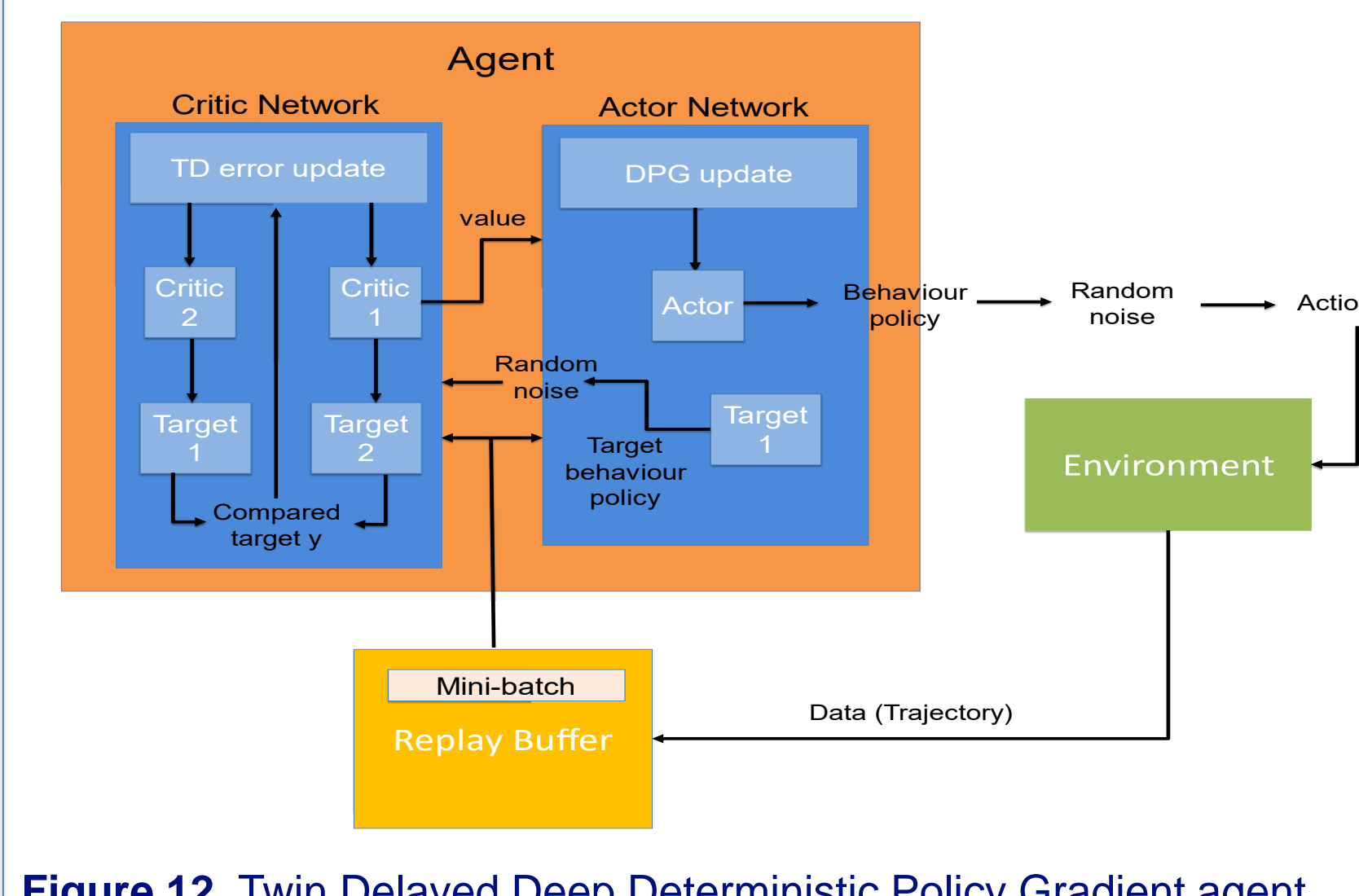
Figure 12. Twin Delayed Deep Deterministic Policy Gradient agent architecture.
