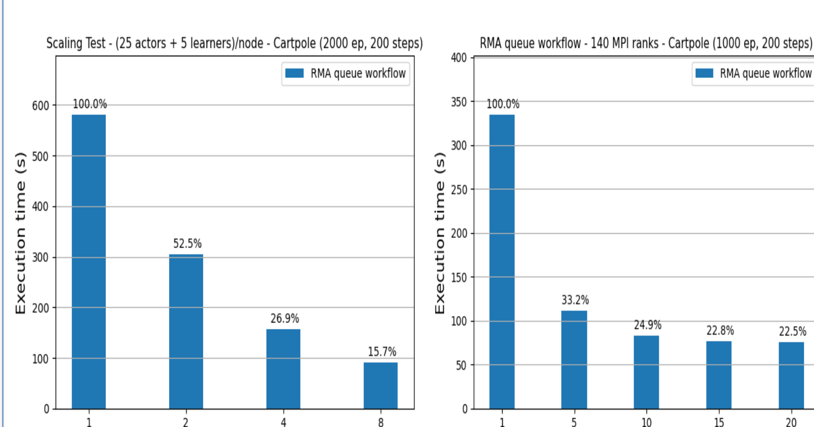
Figure 15. Results for RMA queue scaling
