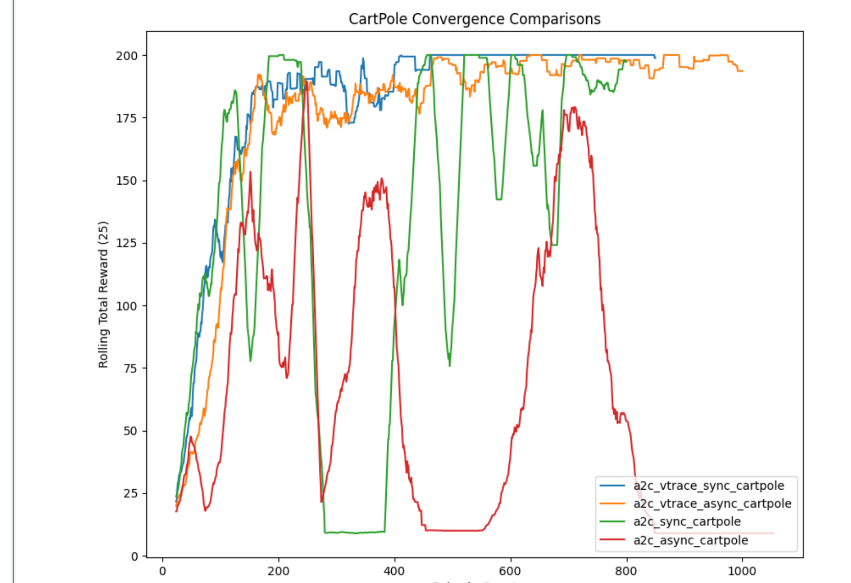
Figure 18. Performance of A2C/A3C with and without v-trace for CartPole environment. Note that A2C/A3C without v-trace does not converge, whilst A2C/A3C with v-trace does.
