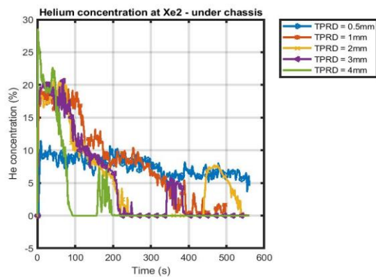
Figure 16. Sensor located under chassis at 1.9m of the TPRD and at
