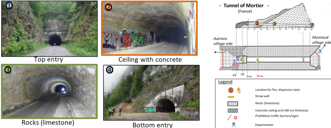
Figure 1. Tunnel geometry
