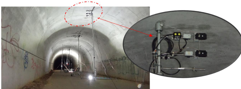
Figure 4. Gas dispersion measurement sensors
