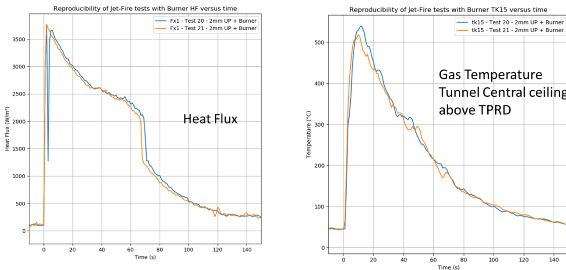
Figure 9. Reproducibility of jet-fire tests.
