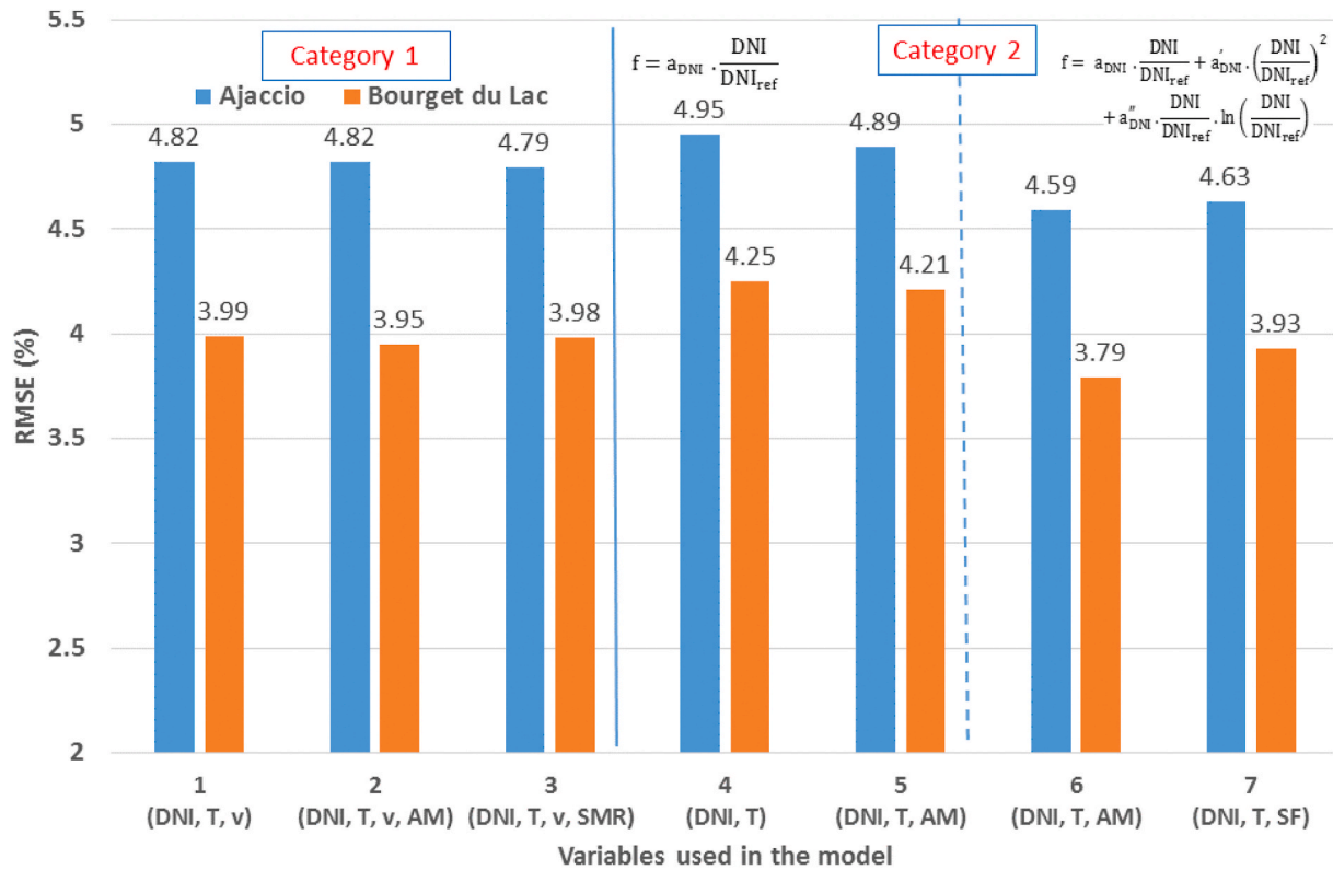
Fig. 8. RMSE value for each model applied on the two sites.
