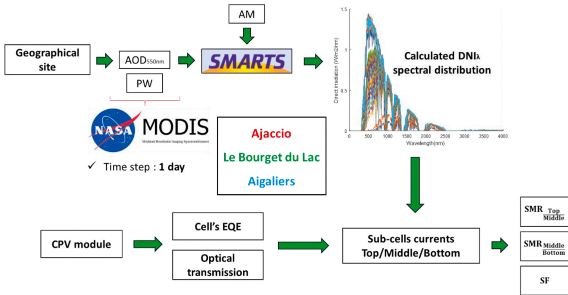
Fig. 5. Estimation of spectral indicators SF and SMR using SMART [18] from AM, PW and AOD 550nm . The External Quantum Efficiency (EQE) of the MJSC is obtained from Refs. [57,59]. Fig. 6 shows the EQE of the GaInP/GaInAs/GaInNAs cells used in the two experimental systems.
