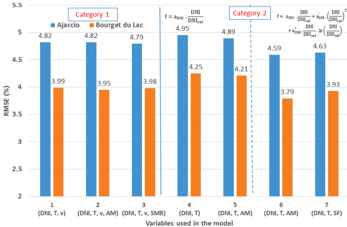
Fig. 8. RMSE value for each model applied on the two sites.
