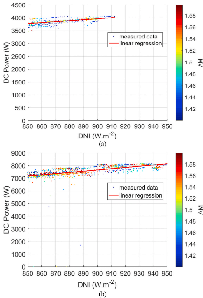
Fig. 9. Measured electrical power around CSOC conditions as a function of DNI with a colour scale of AM in Ajaccio (b) and Le Bourget du Lac (a). (For interpretation of the references to colour in this figure legend, the reader is referred to the Web version of this article.)
