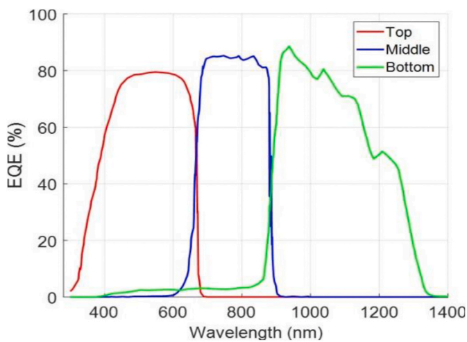
Fig. 6. External Quantum Efficiency of the Semprius cell.
