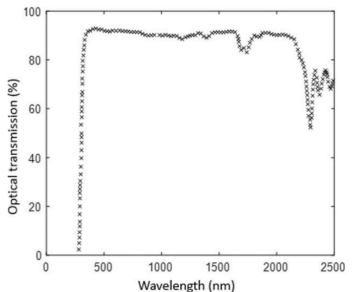
Fig. 7. Optical transmission of the Primary Optical Element in silicon on glass.
