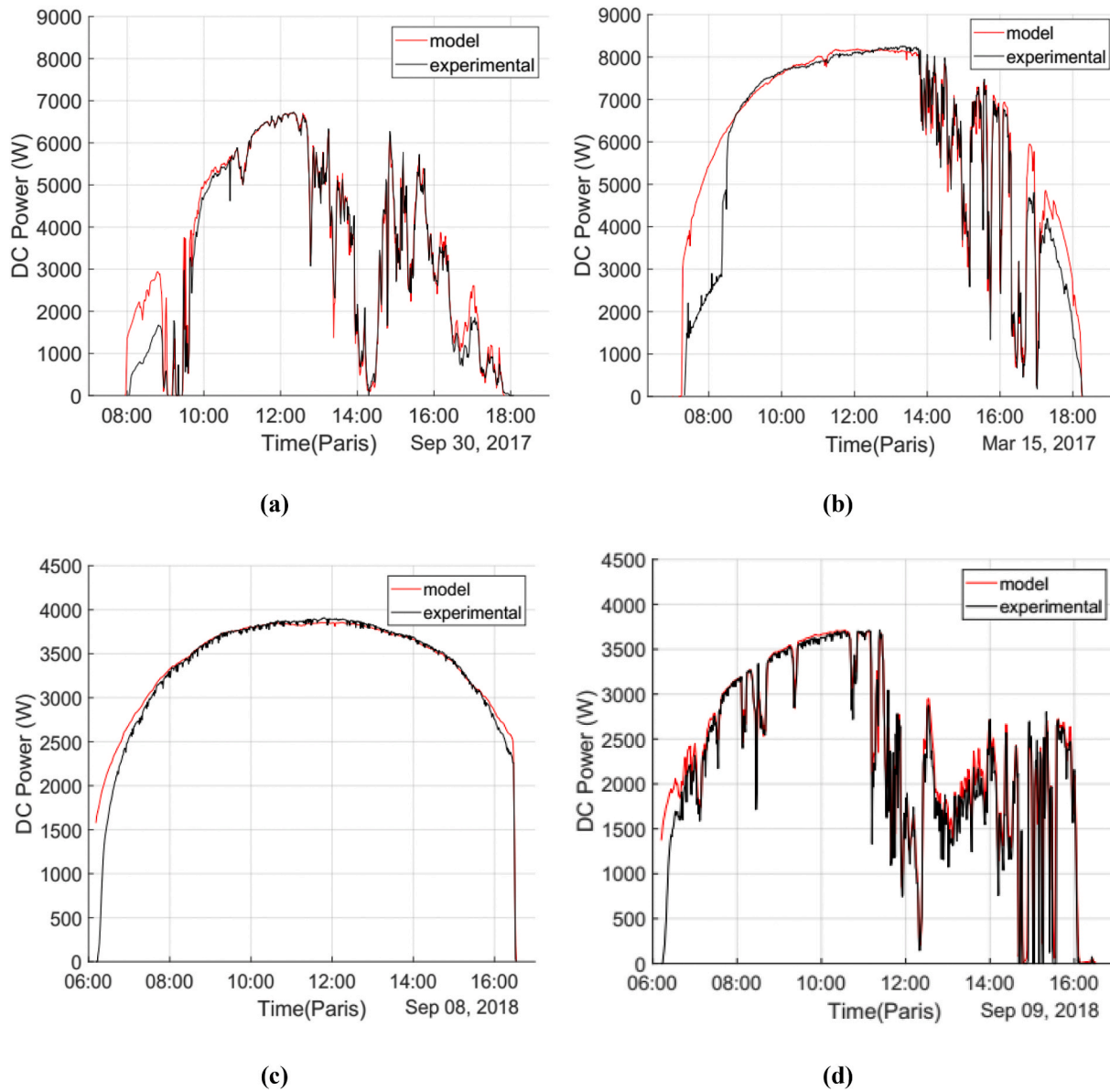
Fig. 10. Experimental validation on Ajaccio (a and b) and Le Bourget du Lac (c and d).
