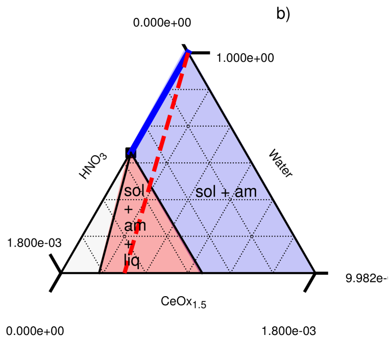
Figure 3: a) scattering efficiency at 250 ms reaction time, from equation 1. (-----) calculated from the phase diagram b) example of a phase diagram compatible with the experimental scattering efficiency.
