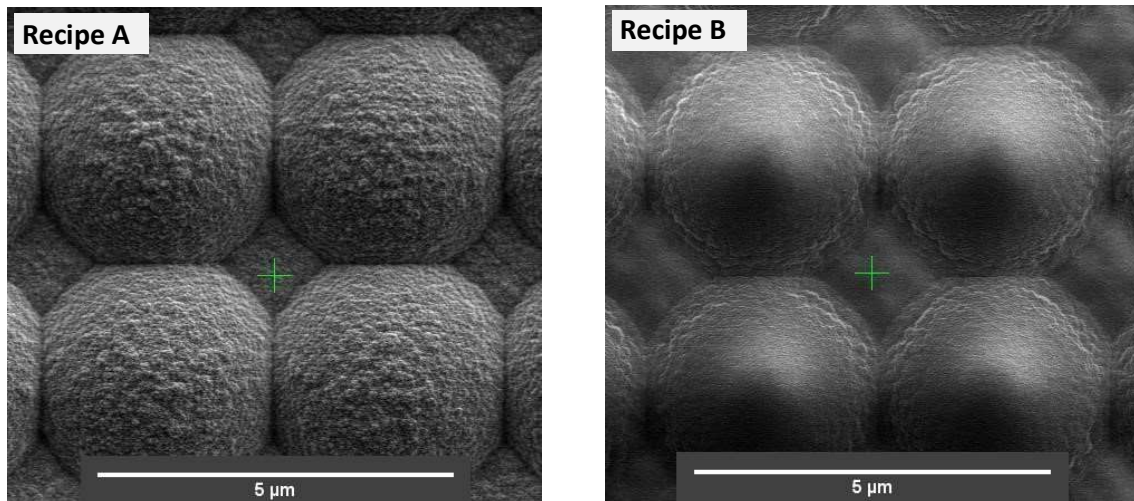
Figure 2. SEM images of etched microlenses showing roughness and shape modification. Recipe A: \text{NF}_3/\text{C}_4\text{F}_8/\text{CF}_4 . Recipe B: \text{CF}_4 .
