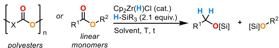
Scheme 2. Development of a general procedure for Zr-catalysed ester hydrosilylation.
