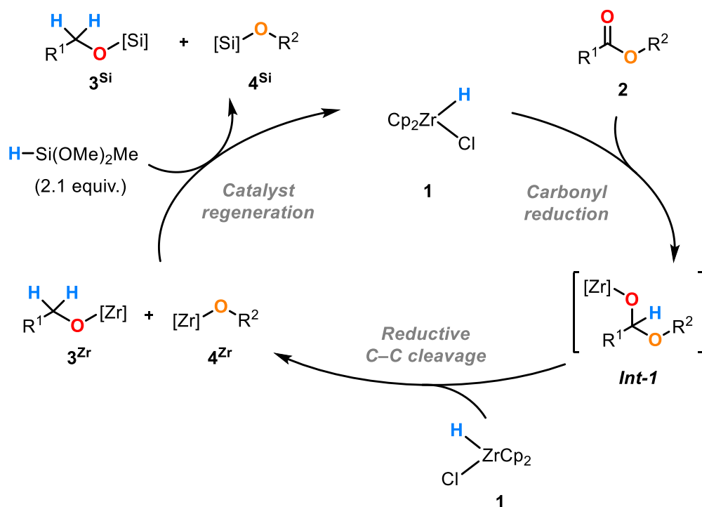
Scheme 3. Proposed catalytic cycle for the reduction of esters 2 by complex 1 .
