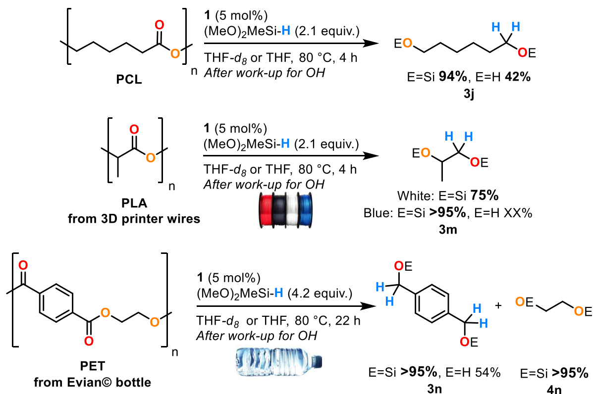
Scheme 5. Reductive depolymerisation of polyesters catalysed by complex 1 . The yields of silyl ethers were measured by ^1\text{H} NMR spectroscopy by integration against mesitylene as an internal standard (reactions conducted in \text{THF-}d_8 ). The yields of alcohols are isolated yields from reactions in THF after basic workup.
