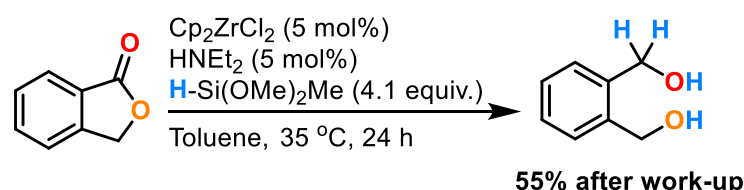
Scheme 1. Limited previous examples of ester reduction mediated/catalysed by Zr-H.
