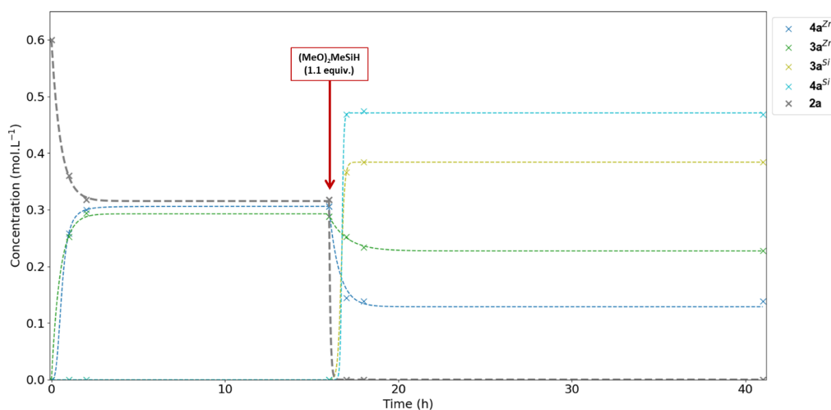
Figure 1. Time-step analysis by ^1H NMR spectroscopy of the stepwise stoichiometric reduction of 2a by complex 1 and DMMS.
