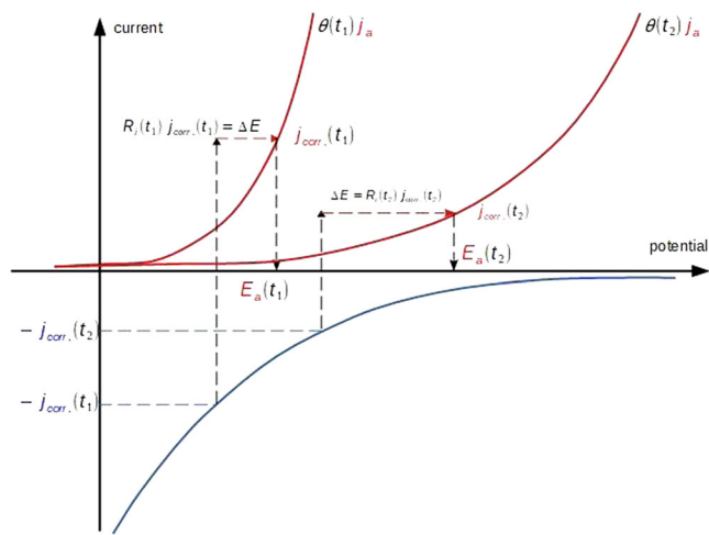
FIGURE 14 Coupling between the anodic and cathodic Butler-Volmer current-voltage curves for P285-NH steel. J_a anodic current, E_a anode potential, J_{corr} corrosion current, \Delta E = E_a - E_c , E_c cathode potential, \theta(t_1) > \theta(t_2) electroactive anodic surfaces decreased because of the clogging of iCP.
