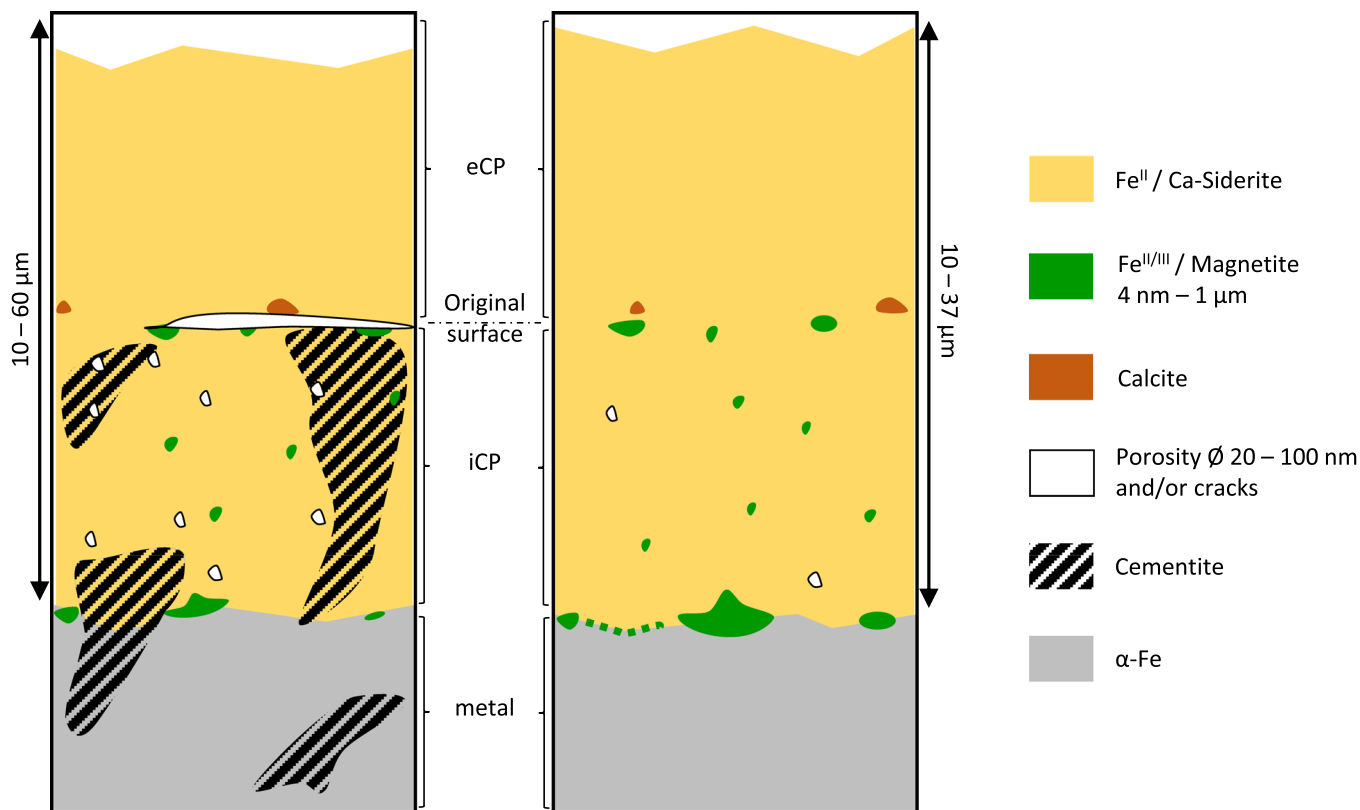
FIGURE 12 Schematic diagram of the corrosion forms observed on (left) the ferrite-pearlitic steel and (right) on the ferritic samples
