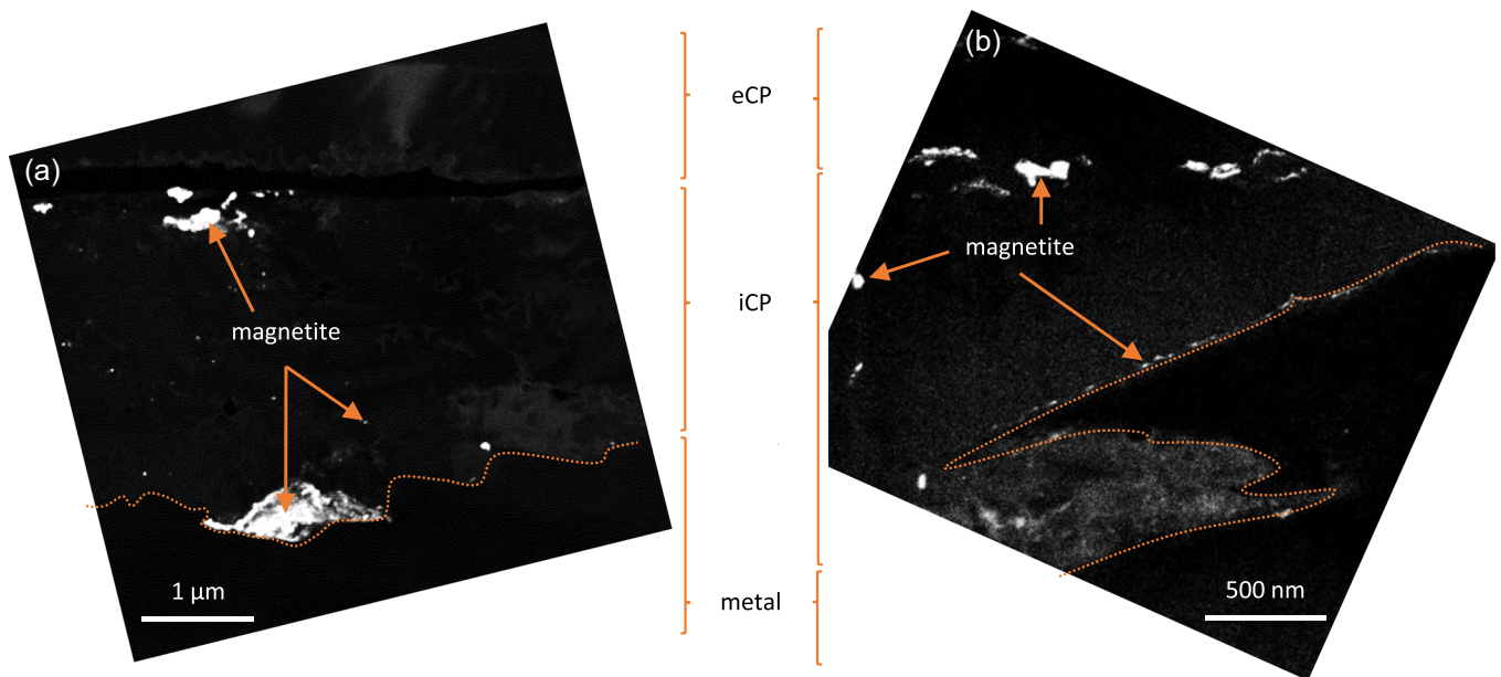
FIGURE 11 Location of nanometric to micrometric islets of magnetite in the corrosion product layer (CPL) of (a) the ferrito-pearlitic and (b) the ferritic samples. The orange discontinuous lines correspond to the M/CPL interface. Darkfield transmission electron microscopy orientation images were obtained by positioning the aperture of the objective on a magnetite diffraction spot.
