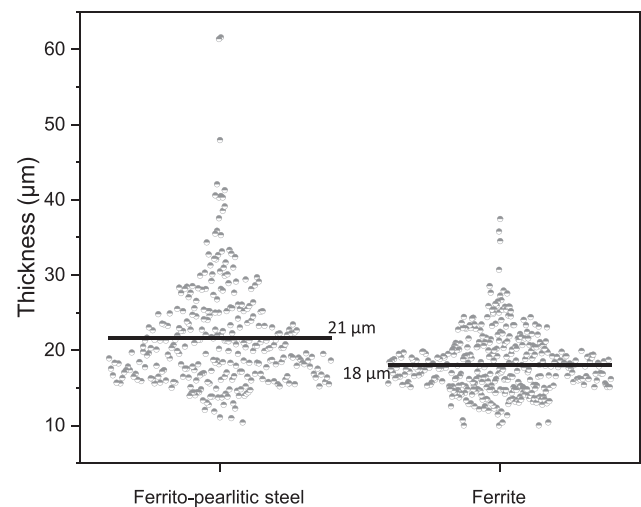
FIGURE 3 Corrosion product layer thicknesses for the ferrito-pearlitic and the ferritic samples. The black line corresponds to the average of the measured values (P285-NH: 311 measurements on 56 images, Armco: 383 measurements on 54 backscattered electron-scanning electron microscopy images).
