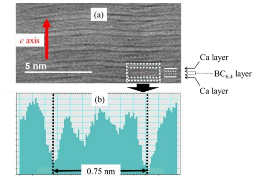
Figure 7. (a) Cross-section image of main part of the Ca intercalated BC_{6.4} film observed with STEM and (b) contrast change image in the direction of c -axis. These indicate the second stage structure 12 .
