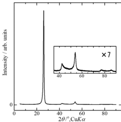
Figure 2. X-ray powder diffraction of B/C/N material ( BC_{2.6}N_{0.55} ).
