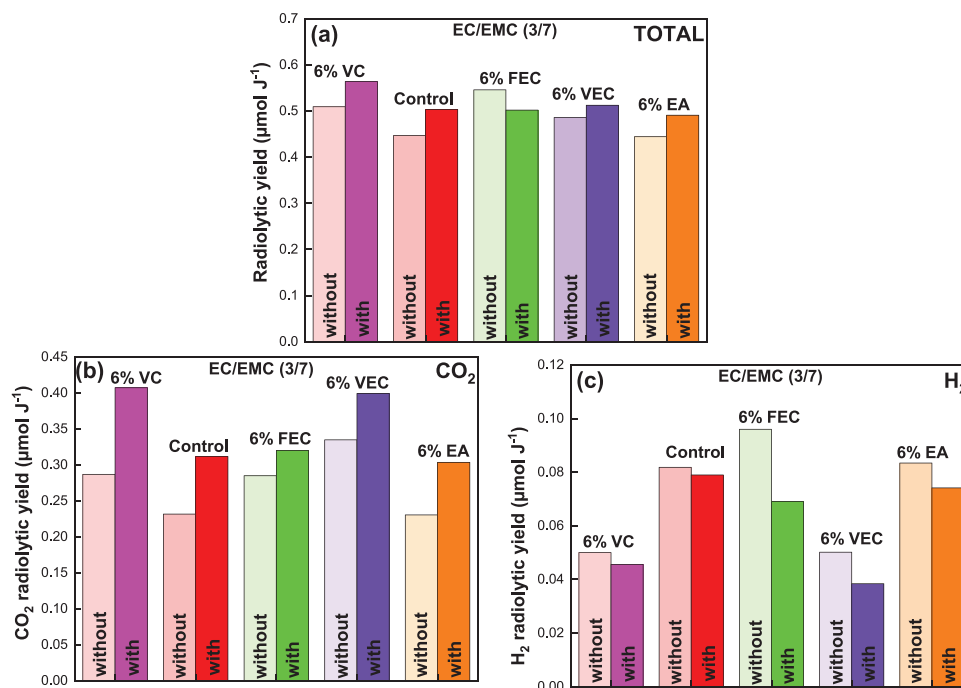
Figure 5. Evolution of radiolytic yields of a) the total of the four gases ( \text{CO}_2 , \text{CO} , \text{H}_2 and \text{CH}_4 ), b) \text{CO}_2 , and c) \text{H}_2 gases produced after irradiation of electrolytes without or with \text{LiPF}_6 at 1 M. The uncertainty is estimated to be 7%.
