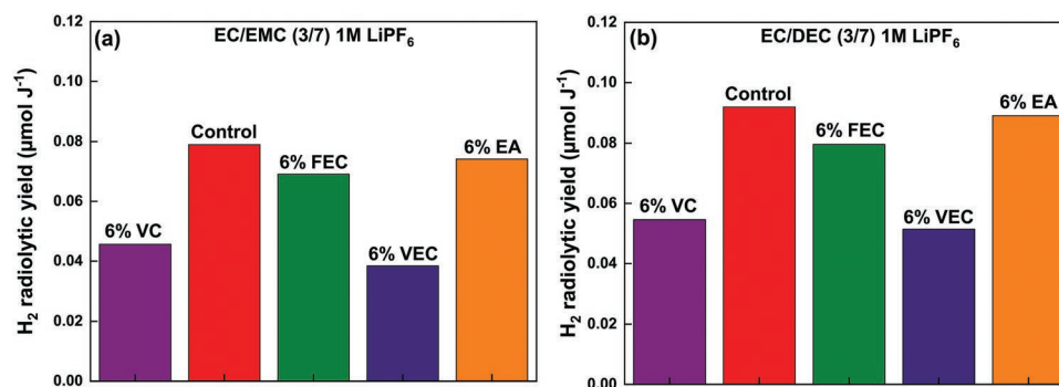
Figure 3. Evolution of the H_2 radiolytic yield for electrolytes containing a) EC/EMC (3/7 v/v) and b) EC/DEC (3/7 v/v) with 1 M \text{LiPF}_6 and various additives. The same color code as in Figure 2 is used. The uncertainty is estimated to be 7%.
