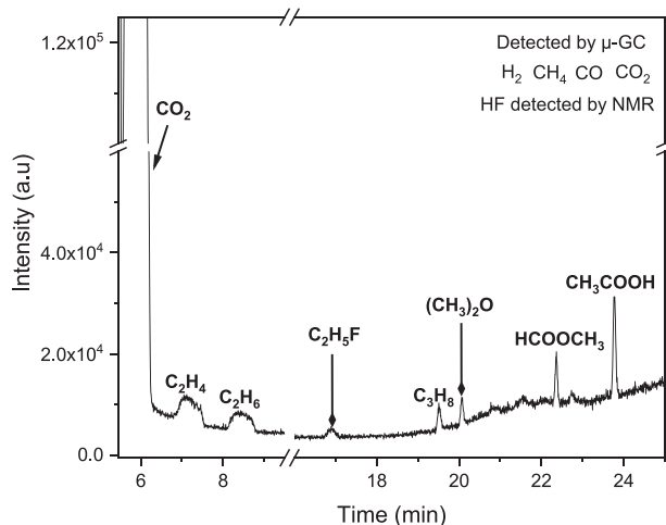
Figure 6. Gas decomposition products of the reference electrolyte (EC:EMC/1 M \text{LiPF}_6 ) were measured by GC/MS after a 6 kGy irradiation. The ( \text{H}_2 , \text{CH}_4 , \text{CO} , \text{CO}_2 ) molecules written on the top, were identified and quantified by \mu\text{-GC} experiments. \text{HF} was detected by NMR. \text{CO}_2 was identified by both \mu\text{-GC} and GC/MS techniques. Other gases were identified by the GC/MS experiment only.
