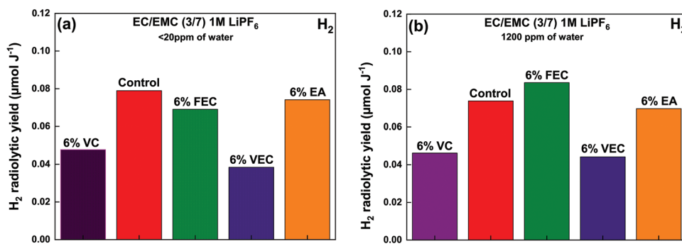
Figure 4. Evolution of the H 2 radiolytic yield for electrolytes EC/EMC (3/7 v/v) with 1 M LiPF 6 and various additives containing a) <20 ppm of water and b) 1200 ppm of water. The same color code as in Figure 2 is used. The uncertainty is estimated to be 7%.
