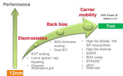
Fig 18: FDSOI boosters and roadmap towards a 7nm node.
