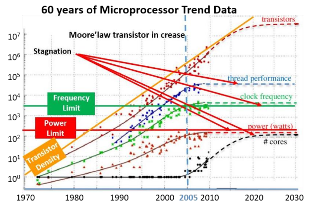
Fig 5: Evolution of processor performance adapted from [14].
