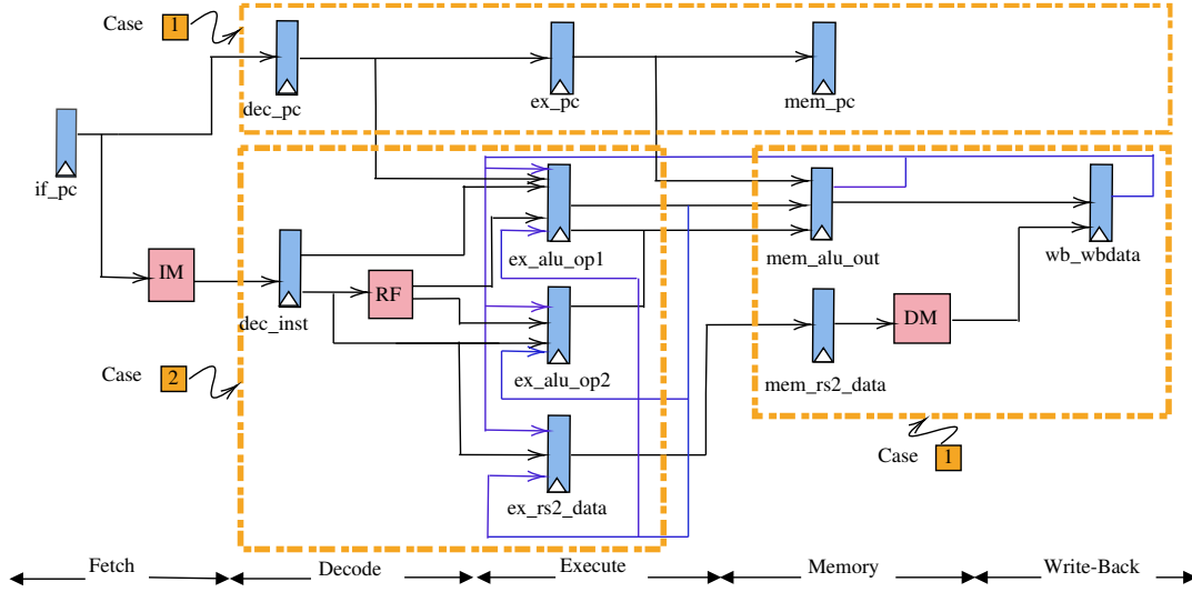
Fig. 2: RISC-V Sodor 5-stages pipeline datapath model.
