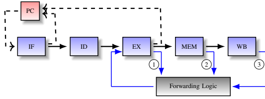
Fig. 1: Classical 5-stage pipeline with forwarding.
