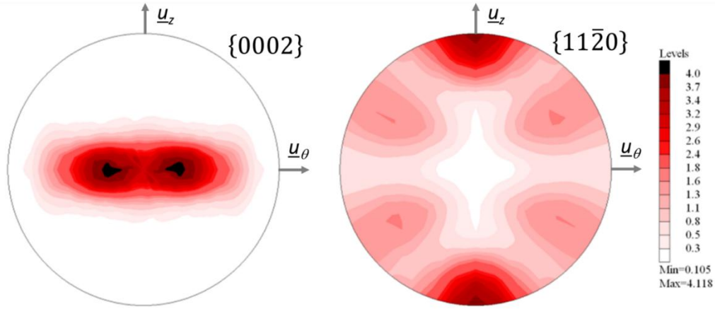
Figure 2: {0002} and {11 \bar{2} 0} pole figures obtained from the XRD texture analysis of the recrystallized Zircaloy-4 guide tube.
