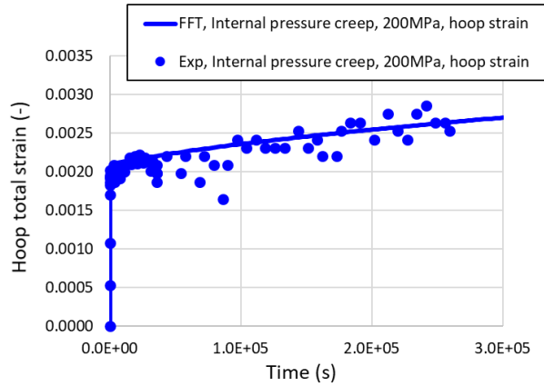
Figure 7: FFT simulations (using Voronoi grains with N=21 , r=5 ) compared to experimental results of a post-irradiation creep test conducted at 350^{\circ}\text{C} on RZA Zy-4, under internal pressure, with applied hoop stress of 200 MPa. The total hoop strain is shown as a function of time.
