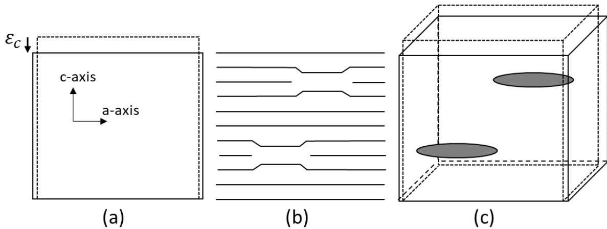
Figure 4: Schematic explaining the origin of the strain along the \langle c \rangle axis during growth acceleration.
