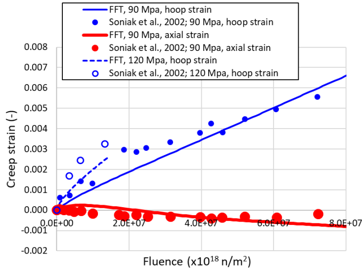
Figure 8: FFT simulations (using Voronoi grains with N=21 and r=5 ) compared to experimental results of internal pressure creep tests conducted on RXA Zy-4 under irradiation at 350^{\circ}\text{C} in materials testing reactor (Soniak et al., 2002). Two tests are reported with an applied hoop stress respectively of 90 MPa and 120 MPa. For the test conducted with an applied hoop stress of 90 MPa, both axial and hoop strain are given (resp. in red and blue).
