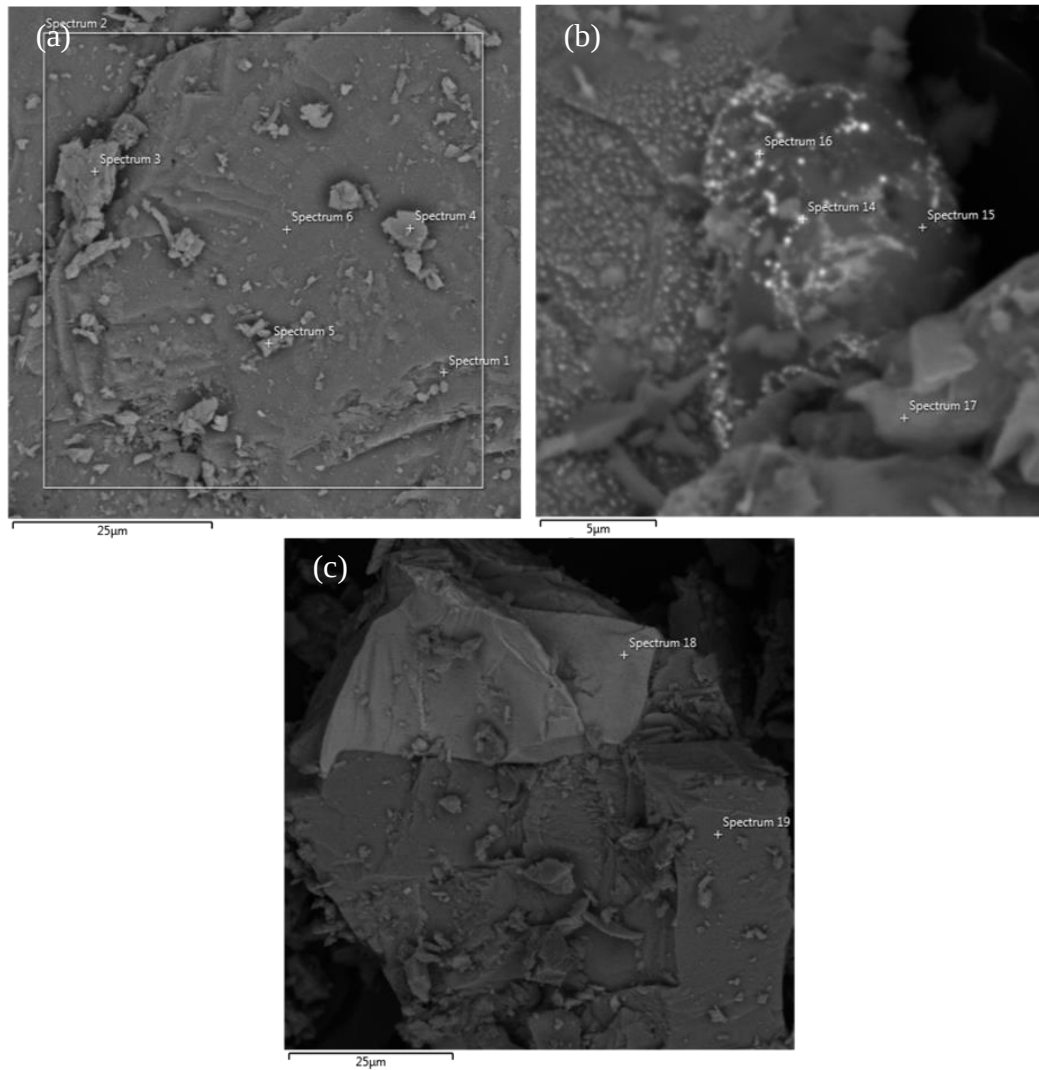
Fig. 5. Cross-sectional images of granites from the Ipojuca River basin using a scanning electron microscope with energy-dispersive X-ray spectroscopy attached facilities (SEM-EDS). A) granite from the upper catchment. B) metaluminous granite from the middle catchment. C) granite from the upper catchment.
