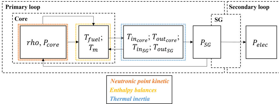
Fig. 7. Schematic of the quantities for the global modelling of the reactor.
