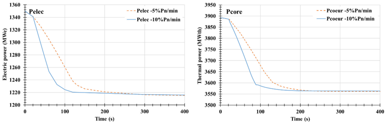
Fig. 11. Electrical and thermal power for a constrained transient at -10\%P_n/\text{min} .
