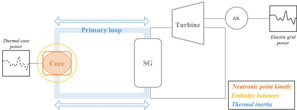
Fig. 6. Diagram of the simplified modelling of a 1300 MW PWR type reactor.
