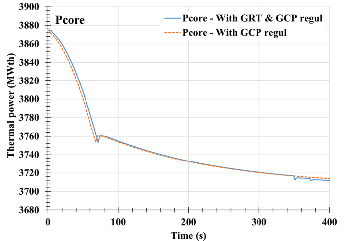
Fig. 5. Thermal core power during load following according to the activated regulation.
