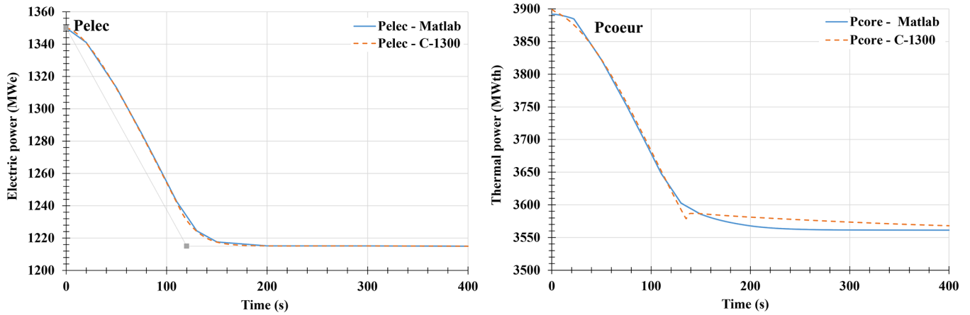
Fig. 8. Electrical and thermal power for the Matlab load-following validation case.
