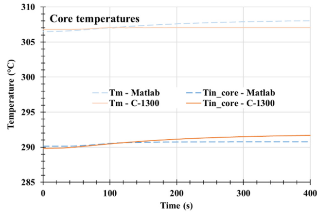
Fig. 10. Comparison of core temperatures for the grid-following validation case.
