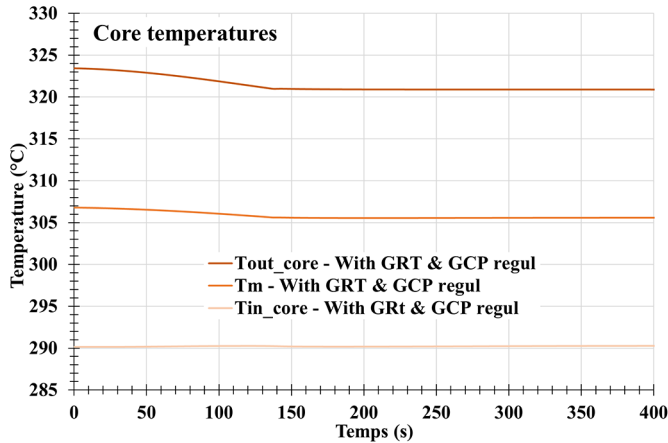
Fig. 4. Temperatures in the core (inlet T_{in\_core} , outlet T_{out\_core} and average T_m ) during a load following transient.
