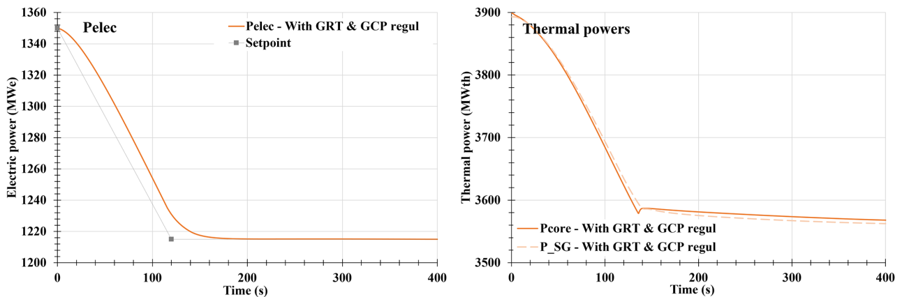
Fig. 3. Electrical and thermal powers (core P_{core} and steam generator P_{SG} ) during a load following transient.
