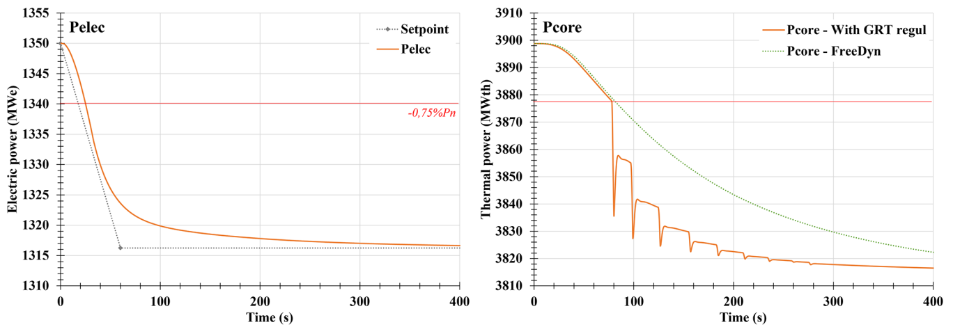
Fig. 1. Electrical and thermal powers during a primary frequency control transient.
