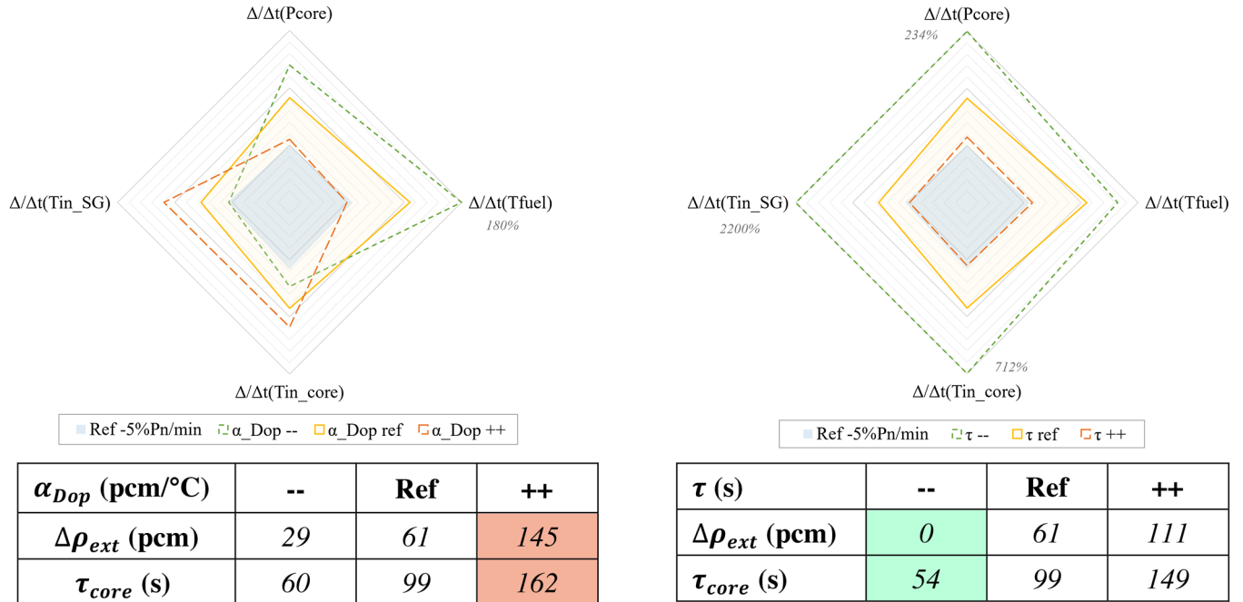
Fig. 13. Radars for the sensitivity study according to both studied parameters.
