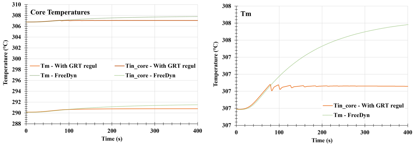
Fig. 2. Temperatures in the core including the average temperature in the core ( T_m ) and inlet core temperature ( T_{in\_core} ) during a primary frequency control transient.
