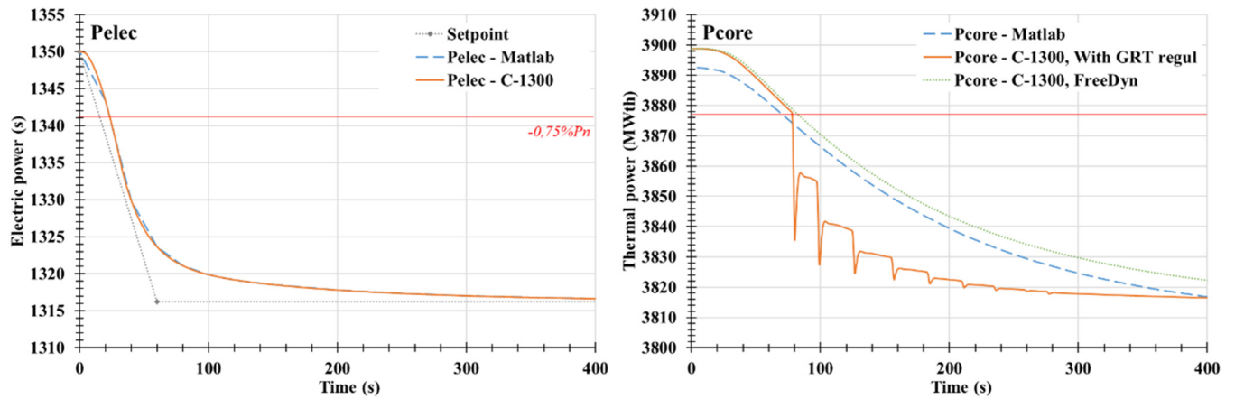
Fig. 9. Comparison of electrical and thermal power for the grid-following validation case.
