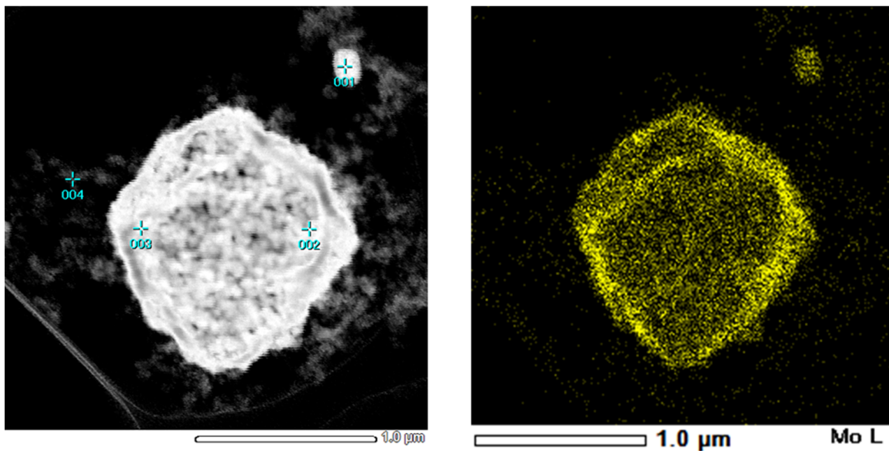
Figure 4. STEM (left) and EDX (right) mapping images of a single MOC10 aggregate. Mo appears in yellow color.
