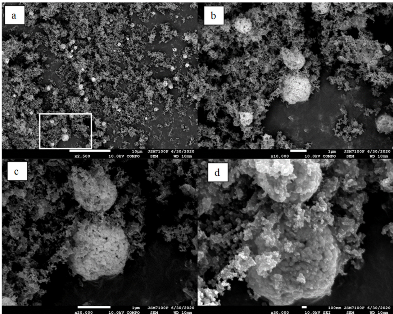
Figure 2. (a–d) Examples of SEM images of MOC10 nanocomposites. Scale bar sizes: (a) 10\ \mu\text{m} , (b) 1\ \mu\text{m} , (c) 1\ \mu\text{m} , (d) 100\ \text{nm} .
