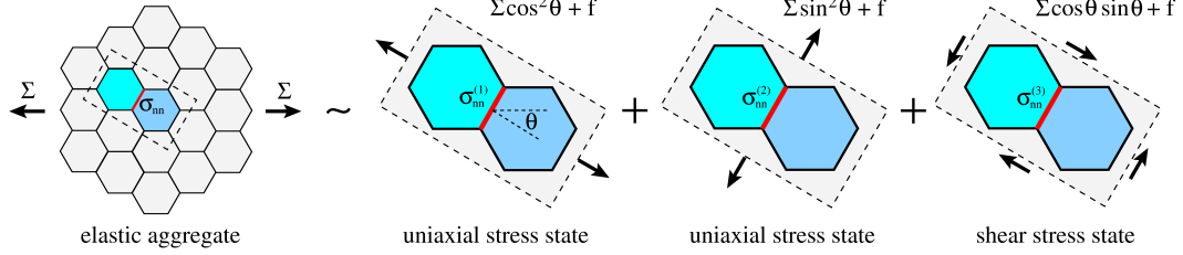
Figure 8. A 2D bicrystal model embedded in elastic aggregate under macroscopic tensile stress \Sigma . To estimate the local stress acting on the bicrystal neighborhood, the macroscopic stress tensor is first dressed up with fluctuations ( f ) to account for the anisotropy of far-field grains, then rotated onto a GB plane by angle \theta and finally rewritten as a superposition of three simpler cases: two with a uniaxial and one with a shear stress state (with 2D stress amplitudes denoted above). In 3D the same stress decomposition would provide three uniaxial and three shear stress states, with the amplitude of the uniaxial stress mode acting along the GB normal being the same as in 2D, namely \Sigma \cos(\theta)^2 + f . Following the principle of linearity, the solution for INS is obtained as a sum of the three partial solutions, \sigma_{nn} = \sigma_{nn}^{(1)} + \sigma_{nn}^{(2)} + \sigma_{nn}^{(3)} .
