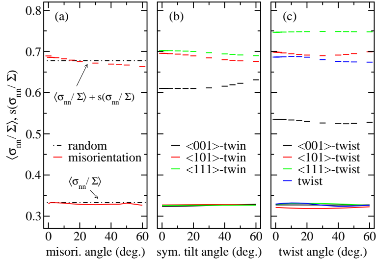
Figure 5. Mean value and standard deviation of normalized INS, \langle \sigma_{nn}/\Sigma \rangle and s(\sigma_{nn}/\Sigma) , plotted as a function of (a) misorientation angle specifying misorientation GBs, (b) symmetric tilt angle specifying \langle abc \rangle -twin GBs, and (c) twist angle specifying \langle abc \rangle -twist and twist GBs. Same Voronoi aggregate model composed of \gamma -Fe grains and under tensile stress \Sigma is used in all calculations. Dashed lines in (a) denote values obtained in the same aggregate but with purely random GBs.
