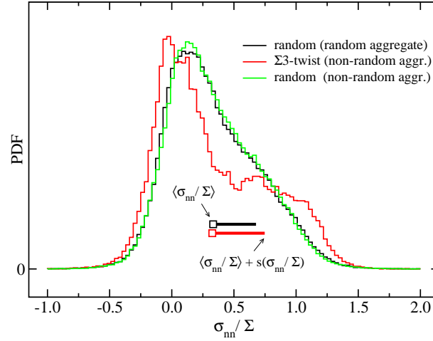
Figure 2. Probability density functions (PDF) of normalized INS \sigma_{nn}/\Sigma calculated in two geometrically equivalent Voronoi aggregate models composed of \gamma -Fe grains under tensile stress \Sigma . A comparison is shown between an aggregate with purely random GBs and an aggregate with 17% GB area corresponding to \Sigma 3-twist GBs (and the remaining 83% GB area to random GBs). In the former case, the distribution is calculated on all GBs, whereas in the latter case two distributions are calculated on either \Sigma 3-twist GBs or random GBs (due to poorer statistics PDF of \Sigma 3-twist GBs is less smooth). To characterize the distributions, the corresponding mean values and standard deviations are depicted on a graph by square symbols and horizontal error bars.
