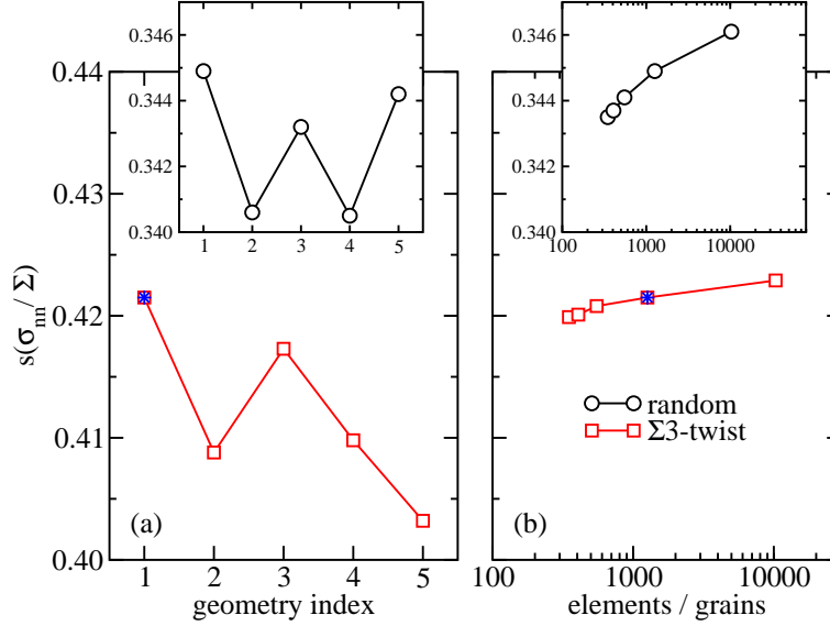
Figure B.15. Standard deviation of normalized INS s(\sigma_m/\Sigma) calculated in a 1000-grain Voronoi aggregate on embedded \Sigma 3 -twist GBs (17% GB area fraction) as a function of (a) grain topology and (b) finite element mesh density. The aggregate used in the main study is marked with star symbol. Insets show similar comparisons for the same aggregates but with purely random GBs. Material properties of \gamma -Fe were used.
