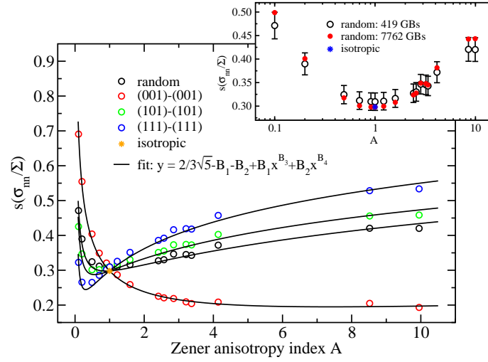
Figure 12. Standard deviation of normalized INS s(\sigma_{nn}/\Sigma) computed on various GB types as a function of Zener anisotropy index A . Results are calculated for all cubic materials from Tab. 1 using either purely random, (001)-(001), (101)-(101) or (111)-(111) GBs (all with 17% GB area fraction) embedded in the Voronoi aggregate model under elastic tensile stress \Sigma . The modelling function shown can be fitted to all four data sets. The inset compares the results obtained in a purely random Voronoi aggregate model when using either 419 GBs (17% GB area fraction) or 7762 GBs (100% GB area fraction) for the calculation of s(\sigma_{nn}/\Sigma) where the isotropic case (denoted by a blue star) serves as a benchmark point. Error bars denote a relative error of 6%, which can be attributed to the statistically smaller sample.
