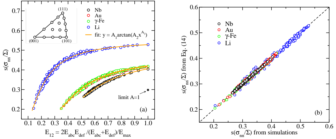
Figure 13. (a) Standard deviation of normalized INS s(\sigma_{nm}/\Sigma) calculated on (abc)-(def) GBs embedded in the Voronoi aggregate model for four selected materials and expressed as a function of effective Young's modulus E_{12} . The modelling function shown can be fitted to all four data sets. In the isotropic limit, A = 1 , the whole E_{12} domain shrinks to a single point at E_{12} = 1 due to orientational invariance of E_{abc} . (b) A comparison of s(\sigma_{nm}/\Sigma) results obtained from finite element simulations and Eq. (14) for four selected materials shown in (a).
