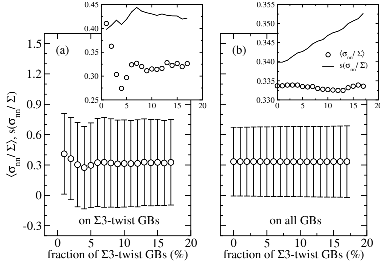
Figure 3. Mean value \langle \sigma_{nn} / \Sigma \rangle and standard deviation s(\sigma_{nn} / \Sigma) of normalized INS, plotted as a function of GB area fraction of \Sigma 3 -twist GBs (with the remaining area fraction corresponding to random GBs). Results in (a) are calculated on \Sigma 3 -twist GBs only and in (b) on all GBs. Insets show the same information but on a different scale. Material properties of \gamma -Fe were used.
