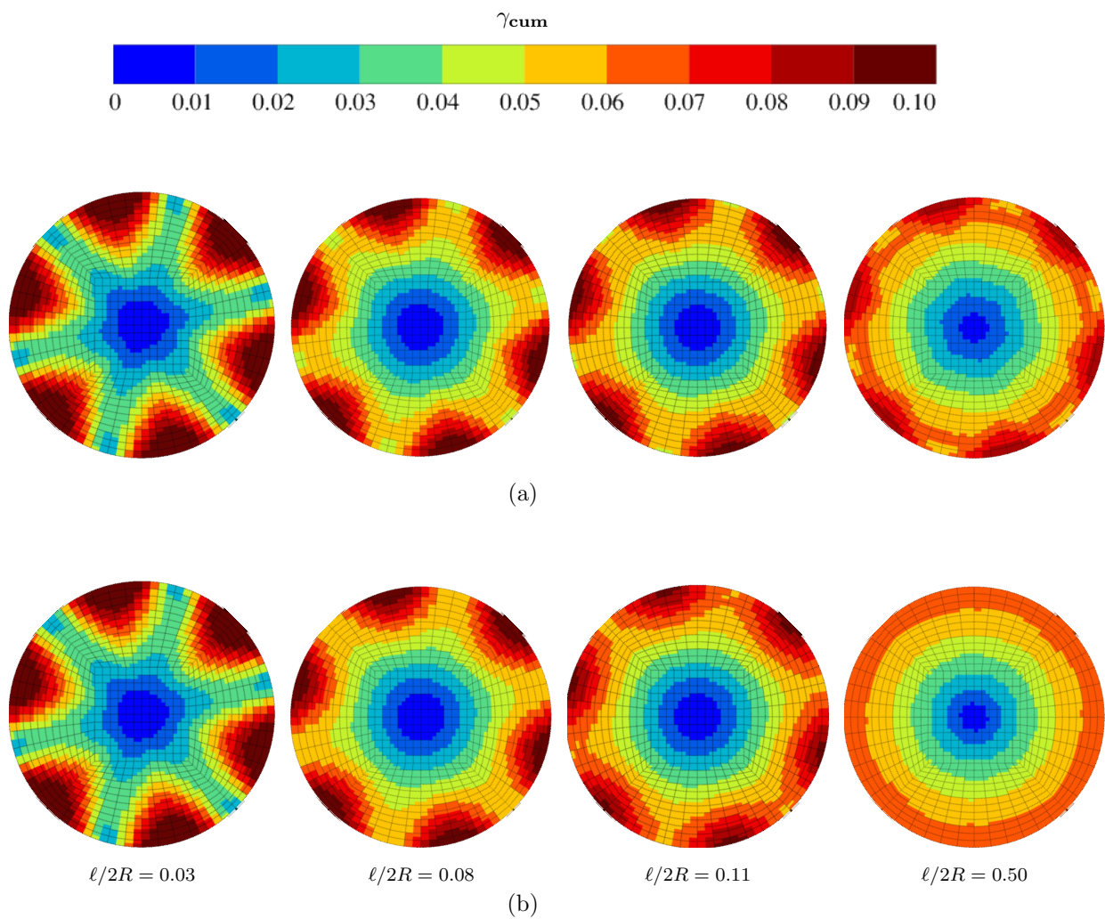
Fig. 9: Cumulative plastic strain distribution in FCC single crystal for \langle 111 \rangle crystal orientation for different values of ratio \ell/2R using (a) micromorphic (b) augmented Lagrangian models at surface strain of 0.08 (fields reported on the reference configuration).
