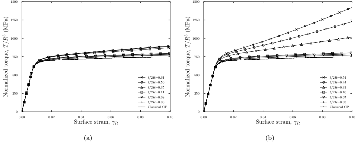
Fig. 11: Normalized torque vs surface strain curves for FCC \langle 111 \rangle crystal orientation for different values of ratio \ell/2R using (a) micromorphic (b) strict strain gradient plasticity model.
