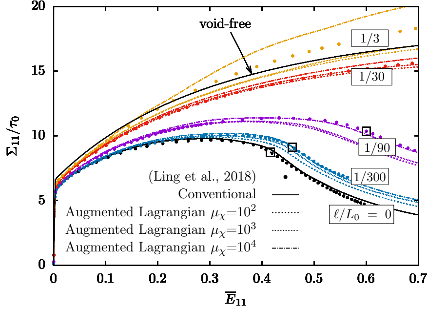
Fig. 15: Macroscopic stress-strain behaviour for different intrinsic length to cell size ratios \ell/L_0 obtained with the micromorphic formulation (dots) by Ling et al. (2018) and the augmented Lagrangian formulation (dashed lines) in porous unit-cell simulations with f_0 = 0.01 and material parameters presented in Table 5. Hollow squares denote onsets of void coalescence.
