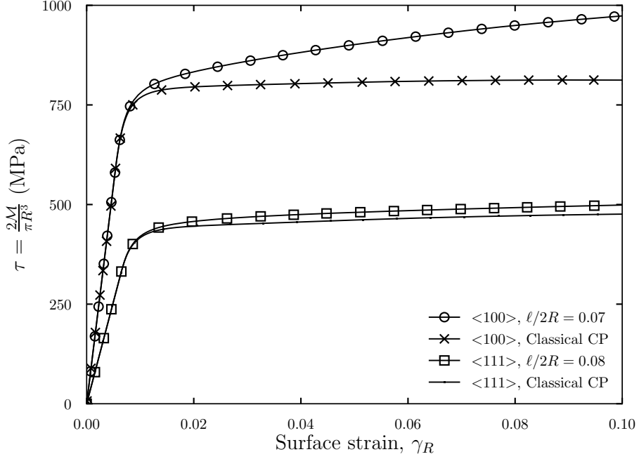
Fig. 7: Shear stress vs surface strain in FCC single crystal wires for \langle 001 \rangle and \langle 111 \rangle crystal orientation using classical crystal plasticity and micromorphic models.
