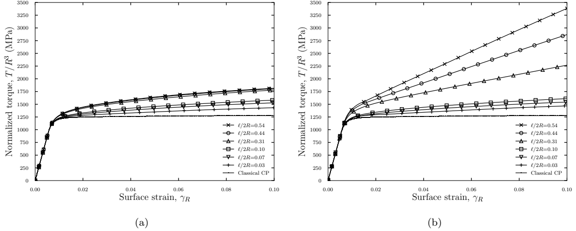
Fig. 10: Normalized torque vs surface strain curves for FCC \langle 001 \rangle crystal orientation for different values of ratio \ell/2R using (a) micromorphic (b) augmented Lagrangian models.
