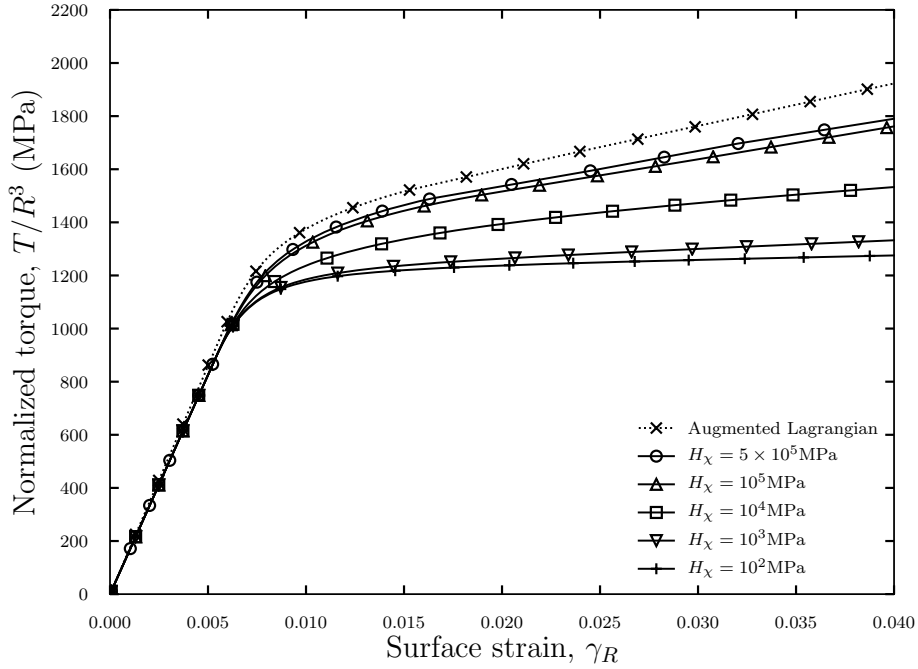
Fig. 12: Normalized torque vs surface strain curves for FCC \langle 001 \rangle crystal orientation for different values of H_\chi and for \ell/2R = 0.44 .
