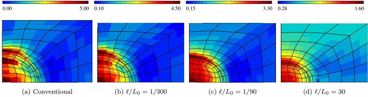
Fig. 16: Cumulated plastic strain fields in porous unit-cells at \bar{E}_{11} = 0.3 obtained with the augmented Lagrangian formulation with \mu_\chi = 10^4 MPa.
