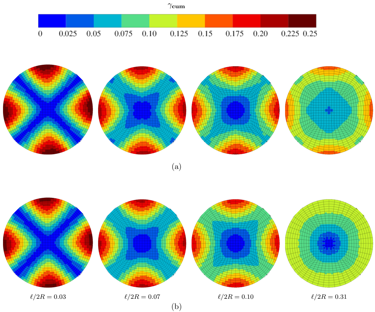
Fig. 8: Cumulative plastic strain distribution in FCC single crystal for \langle 001 \rangle crystal orientation for different values of ratio \ell/2R using (a) micromorphic (b) augmented Lagrangian models at surface strain of 0.08 (fields reported on the reference configuration).
