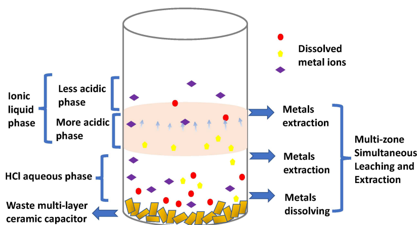
Scheme 2. Simultaneous multi-zone leaching and extraction of valuable metals from waste MLCC by Aliquat ® 336-HCl-H 2 O system.
