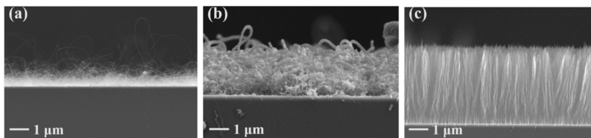
Figure 16. Cross-sectional SEM micrographs of CNT growth on the ZnO film at 800 °C, where: (a) presents the use of pure-thermal CVD in the presence of \text{H}_2 ; (b) or (c) PECVD with \text{H}_2 or \text{NH}_3 , respectively. Reprinted with permission from Yuan, Chemical Physics Letters; Ref. [94] copyright 2021, Elsevier.
