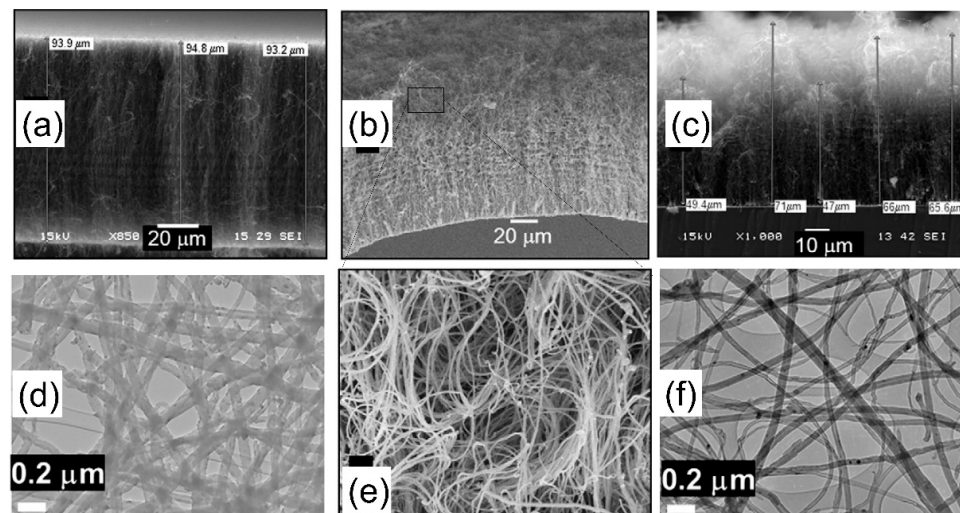
Figure 5. SEM micrographs of CNT carpets on (a) \alpha -Ta(N) at 0.28 N/Ta at.%; (b) Ta 2 N at 1.2 N/Ta at.%; and (c) Ta 5 N 6 at 1.65 N/Ta at.%. (d,f) are the TEM micrographs from CNT recovered from the sample presented in (a,c), respectively; (e) is the SEM magnification of a top part from the CNT carpet presented in (b). All CNT carpets were produced via AACVD at 850 °C by using ferrocene in toluene as carbon precursor. Reproduced with permission from Bouchet-Fabre, Diamond and Related Materials; Ref. [77] copyright 2011, Elsevier.
