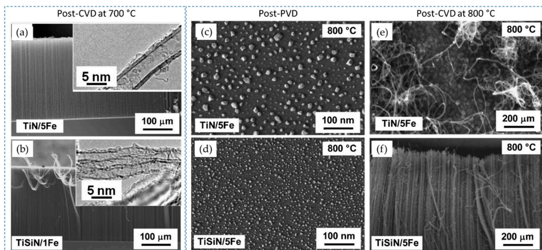
Figure 11. SEM micrographs of VACNT on (a) TiN with 5 nm Fe and (b) TiSiN with 1 nm Fe at 700^\circ\text{C} ; Post-annealing catalyst restructuration on (c) TiN with 5 nm Fe film or (d) TiSiN with 5 nm Fe film at 800^\circ\text{C} , whereas (e,f) present the same after CNT growth at 800^\circ\text{C} , respectively; Reprinted with permission from Yang, physica status solidi (b) basic solid-state physics ; Ref. [89] copyright 2014, John Wiley and Sons.
