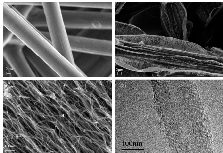
Figure 25. SEM micrographs of (a) before and (b) after growth of VACNT on CF paper coated with catalytic film, whereas (c) presents the VACNT at higher magnification; (d) TEM micrograph of the produced CNT. Reprinted with permission from Zhang, Journal of Physics and Chemistry of Solids; Ref. [123] copyright 2017, Elsevier.
