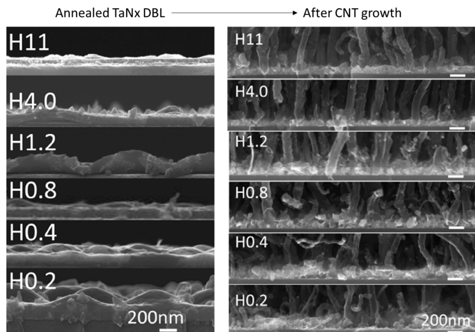
Figure 6. SEM micrographs (left column) for the variation range of TaNx DBLs after annealing under Ar flow and (right column) the same after successive growth of CNT with exposed DBL/CNT interface. Reproduced with permission from Bouchet-Fabre, Applied Surface Science; Ref. [78] copyright 2014, Elsevier.
