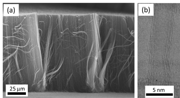
Figure 12. (a) Side-view SEM micrographs of VACNT achieved on TiSiN with 0.4 nm Fe/0.1 nm Al at 600^\circ\text{C} ; (b) HRTEM image of recovered CNT sample; Reprinted with permission from Yang, Applied Physics Letters ; Ref. [90] copyright 2015, AIP Publishing.
