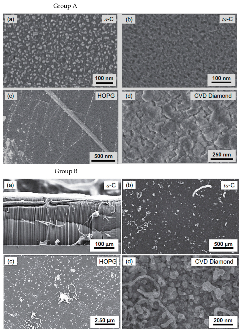
Figure 19. Group A —Top-view micrographs obtained by scanning electron microscopy (SEM) of Fe catalyst nanoparticles deposited on four different sp^2:sp^3 carbons: (a) ( a -C, 85:15 sp^2:sp^3 ), (b) ( ta -C, 30:70 sp^2:sp^3 ), (c) (HOPG, 100:0 sp^2:sp^3 ), and (d) (CVD diamond, 0:100 sp^2:sp^3 ). Group B —idem as in Group A after CVD synthesis of VACNT. Micrographs in Group B —(a) presents cross-section view, whereas (b–d) present top-view. Reprinted with permission from Cartwright, Carbon, Ref. [32] copyright 2014, Elsevier.
