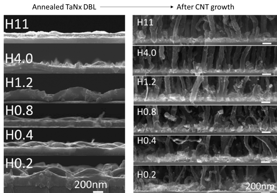
Figure 6. SEM micrographs (left column) for the variation range of Ta x N y DBLs after annealing under Ar flow and (right column) the same after successive growth of CNT with exposed DBL/CNT interface. Reproduced with permission from Bouchet-Fabre, Applied Surface Science; Ref. [78] copyright 2014, Elsevier.
