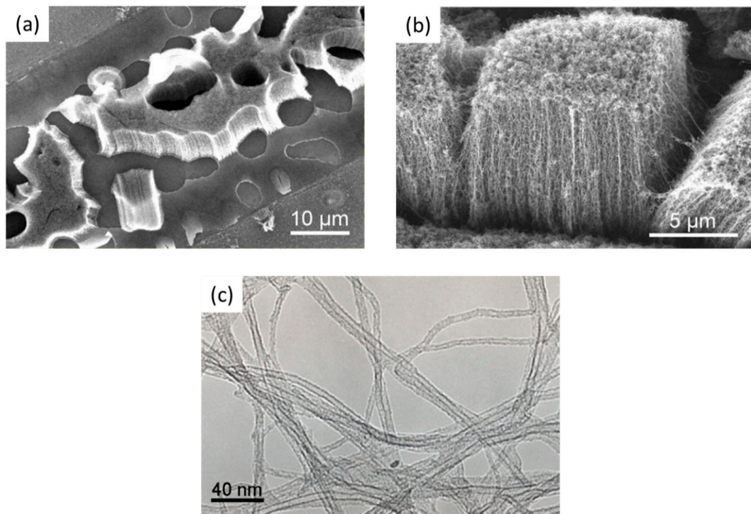
Figure 10. SEM micrographs of (a) the Si/TiN patterned substrate after the AC-CVD synthesis where (b) is the corresponding magnification of a growth zone of VACNT; (c) TEM image of SWCNT selectively grown on TiN surface. Modified after [88].
