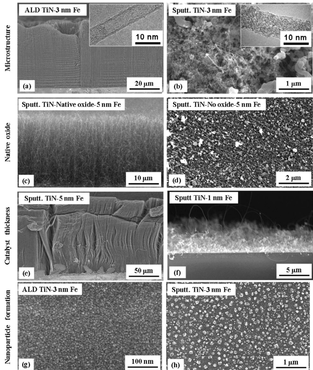
Figure 18. The effect of: (a,b) the microstructure (deposition technique); (c,d) presence of native oxide; catalyst thickness (e,f) over the growth of VACNT presented through a comparison of SEM micrographs. SEM images (g,h) present the density of Fe nanoparticles on DBL formed via the ALD or PVD process, respectively. Idem after growth of VACNT in (a,b). Note that the DBLs, shown (c) or (e), were PVD deposited at 10^{-4} or 10^{-1} mbar and provided different support of VACNT, respectively. Reprinted with permission from S.Esconjauregui, Carbon; Ref. [86] copyright 2014, Elsevier.
