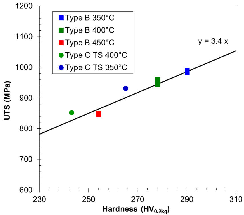
Figure 17: Irradiated CWSR Zircaloy-4 ultimate tensile strength (UTS) during ring tensile test at room temperature after Type B and Type C TS treatment at the lowest studied effective stress versus hardness.
